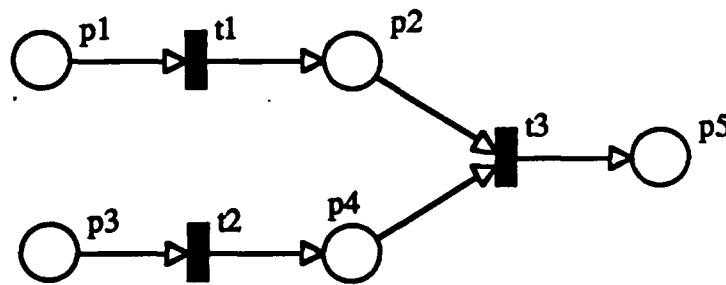
Fig. 2.1 Ordinary Petri Net
