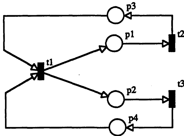
Fig. 2.5 Petri Net P
