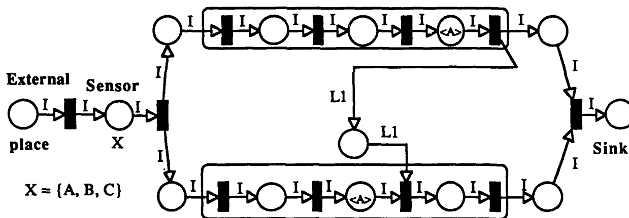
Fig. 5.2 Colored Petri Net with Marking
