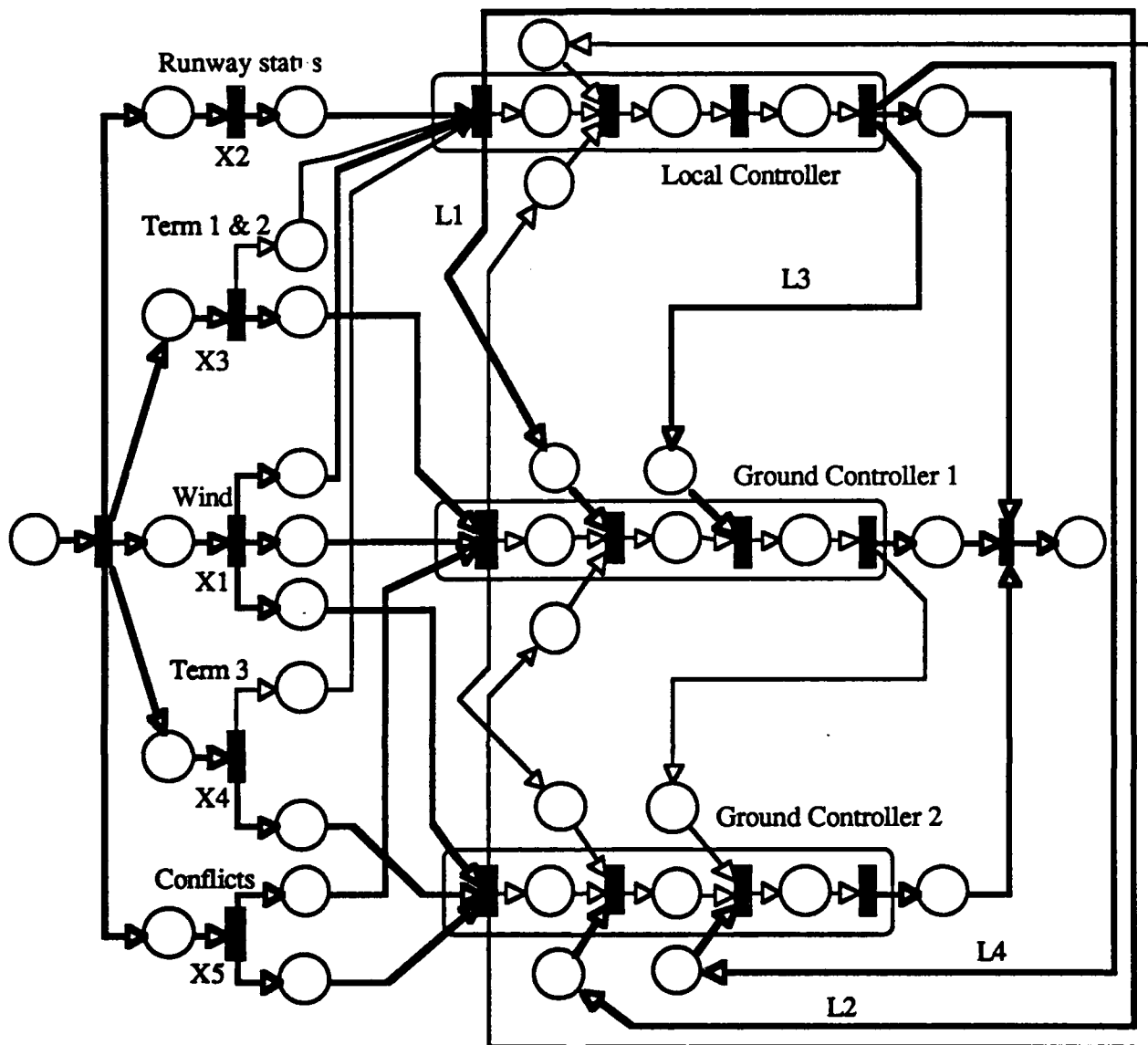
Fig. 8.16 Colored Petri Net model of the Constraints
