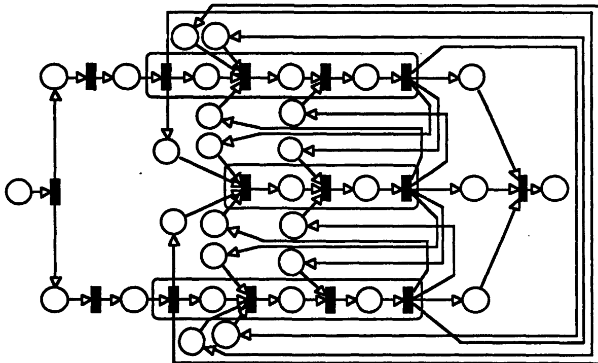
Fig. 8.3 Universal Net for Submarine Example
