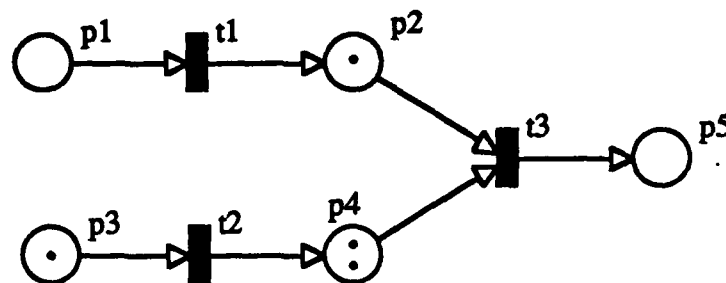
Fig. 2.3 Petri Net after Firing
