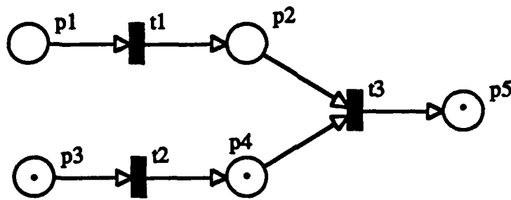
Fig. 2.4 Petri Net after second Firing
