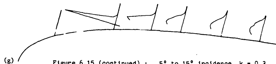
Figure 6.15 (continued) : 5^\circ to 15^\circ incidence, k = 0.3
