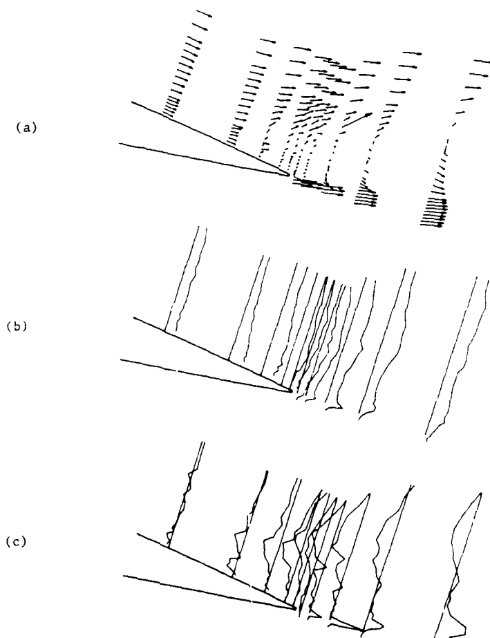
Figure 6.29 : 8^\circ to 18^\circ incidence, k = 0.3
