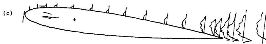
Figure 6.18 : 5^\circ to 15^\circ incidence, k = 0.3
