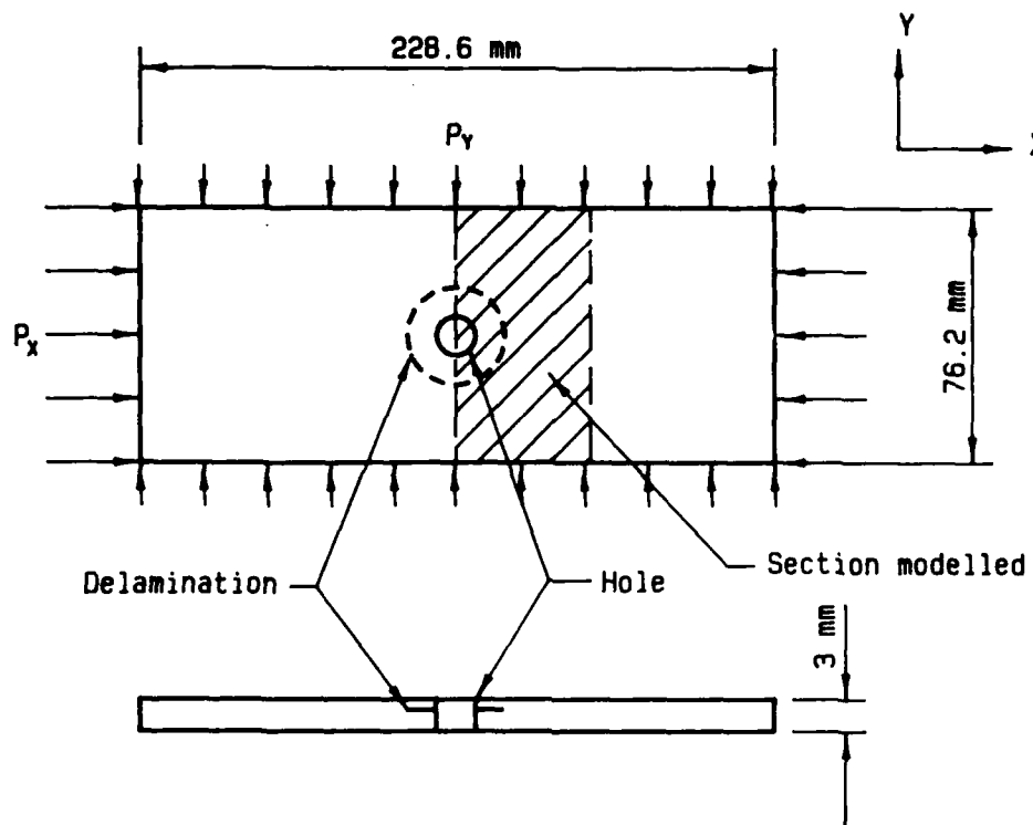
FIG 1: DAMAGED HOLE STRUCTURE.
