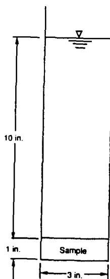
Figure 16 Permeability device.
