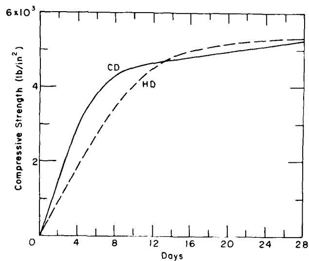
Figure 12. Comparison of strength gain for high-speed and drum-mixed dense concrete.
