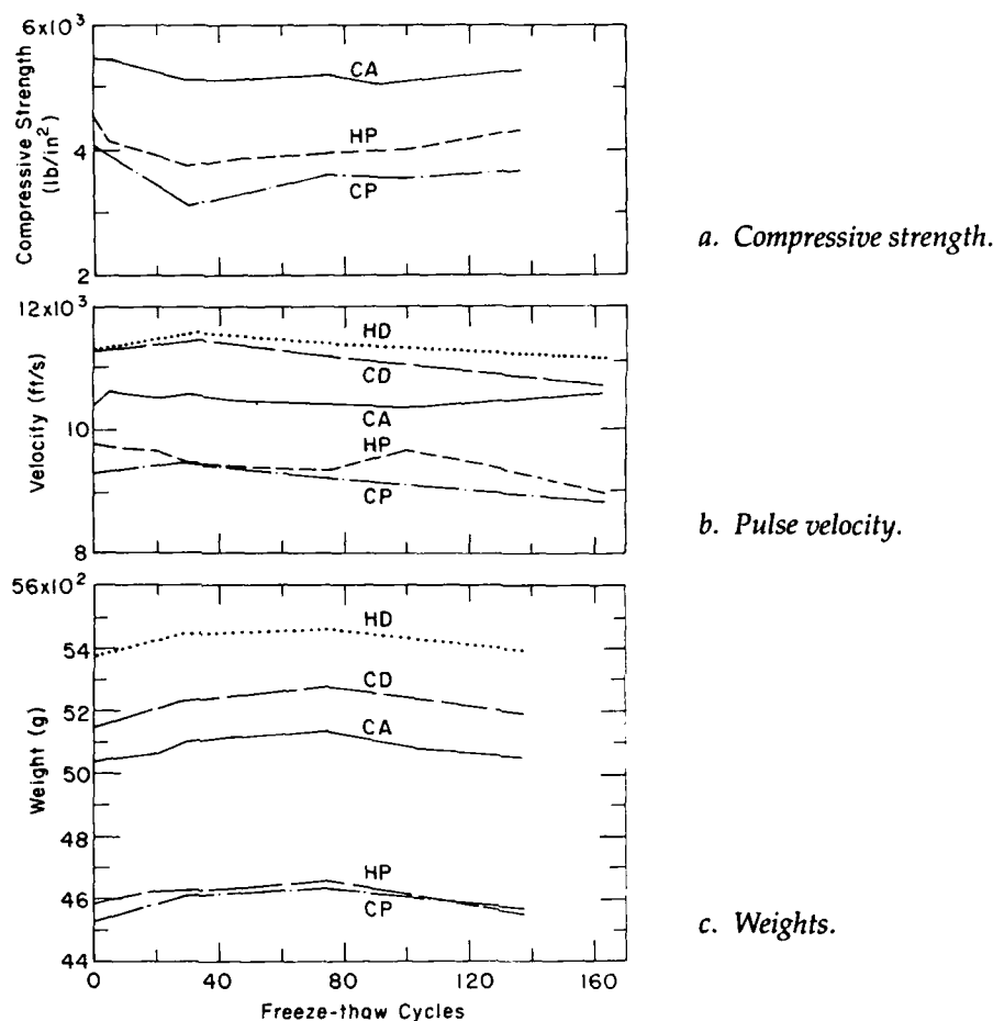
Figure 8. Air-air freeze-thaw test results.
