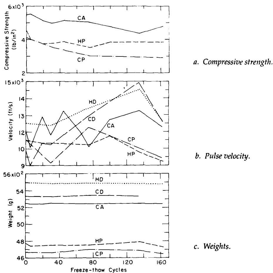
Figure 9. Air-water freeze-thaw test results.
