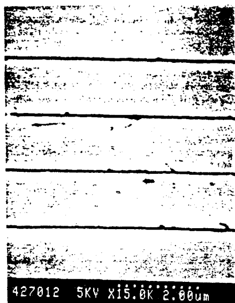
FIG. 7. Patterns in 50-nm Cr film with 14.3-nm LB PMMA as resist, exposed with a high-resolution lithography system at 40-kV accelerating voltage, 12-nm beam diameter, 3-pA beam current and with a dose of 100 \mu\text{C}/\text{cm}^2 . The lines etched in 50-nm-thick Cr are 72 nm wide.
