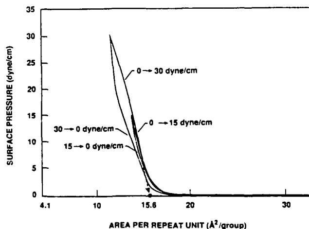
FIG. 2. Pressure-area isotherm for poly(methylmethacrylate) at 20 °C.
