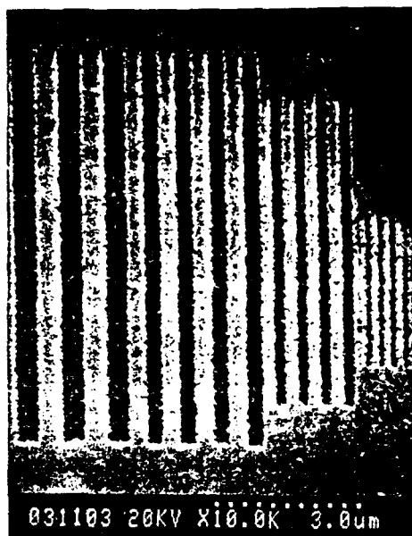
FIG. 5. Patterns in 50-nm Cr film with 14.3-nm LB PMMA as resist, exposed with a MEBES I system at 10 kV accelerating voltage, \frac{1}{4} - \mu\text{m} beam diameter and address size, 6-nA beam current, and with a dose of 30 \mu\text{C}/\text{cm}^2 .
