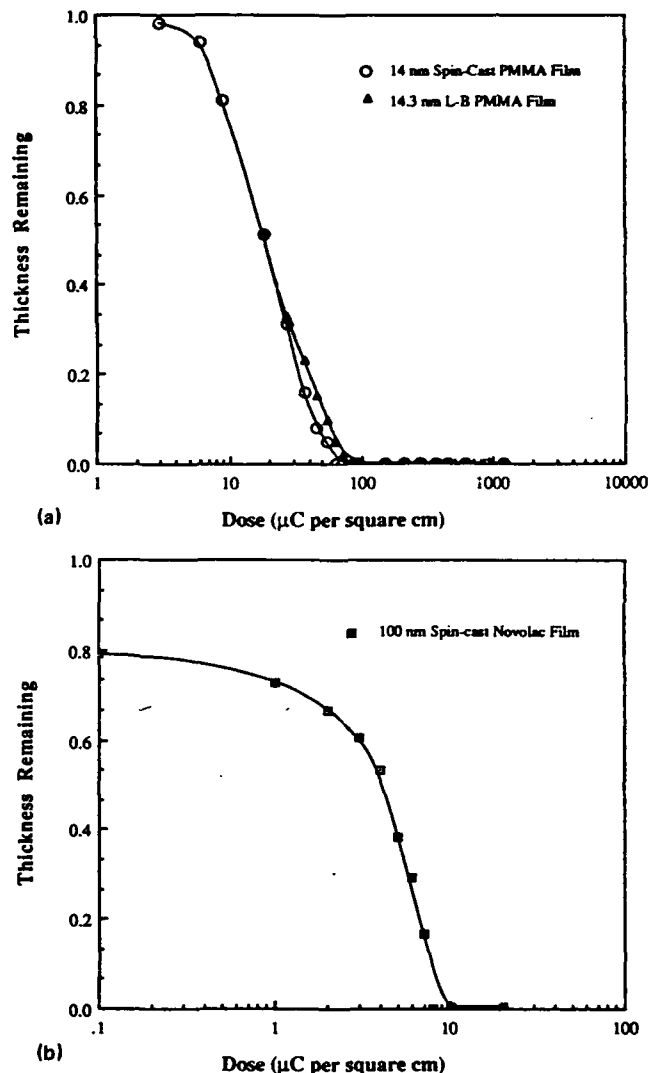
FIG. 3. (a) Characteristic exposure curves of ultrathin PMMA films. (b) Characteristic exposure curve for spin-cast novolac film.
