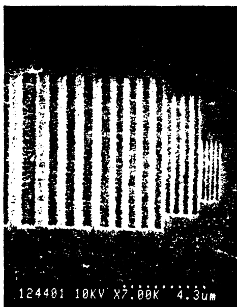
FIG. 4. Patterns in 50 nm Cr with 14 nm spin cast PMMA film as positive e-beam resist, exposed with a MEBES I system at 10 kV accelerating voltage, \frac{1}{4} \mu\text{m} beam diameter and address size, 6-nA beam current, and with a dose of 200 \mu\text{C}/\text{cm}^2 .
