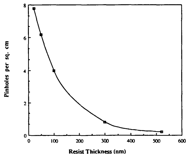
FIG. 8. Pinhole density in 80-nm chromium films after 60-s etching masked by spin-cast AZ 5206 resist films of various thickness. The measurement was done by scanning chromium-on-glass wafers under an optical microscope with a transmitted light illumination.
