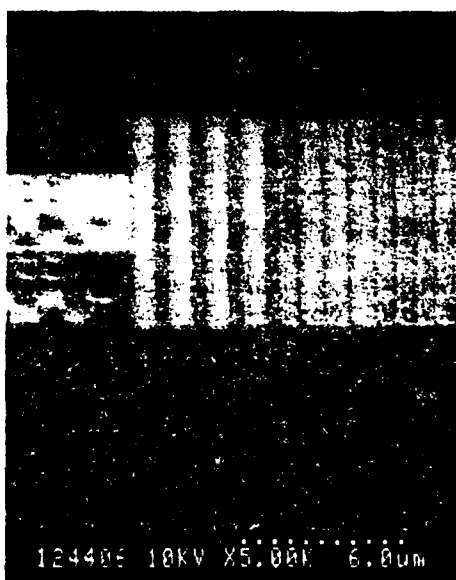
FIG. 6. Overetched pattern in 50-nm Cr film with 22 nm spin cast novolac resist as a positive e-beam resist, exposed with a MEBES I system at 10 kV accelerating voltage, \frac{1}{4} - \mu\text{m} beam diameter and address size, 6-nA beam current, and with a dose of 10 \mu\text{C}/\text{cm}^2 .
