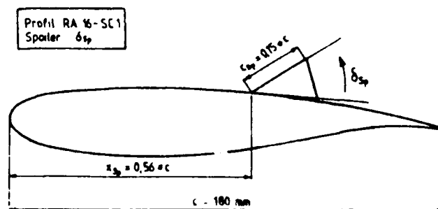
Figure 1. Super critical airfoil with spoiler.
