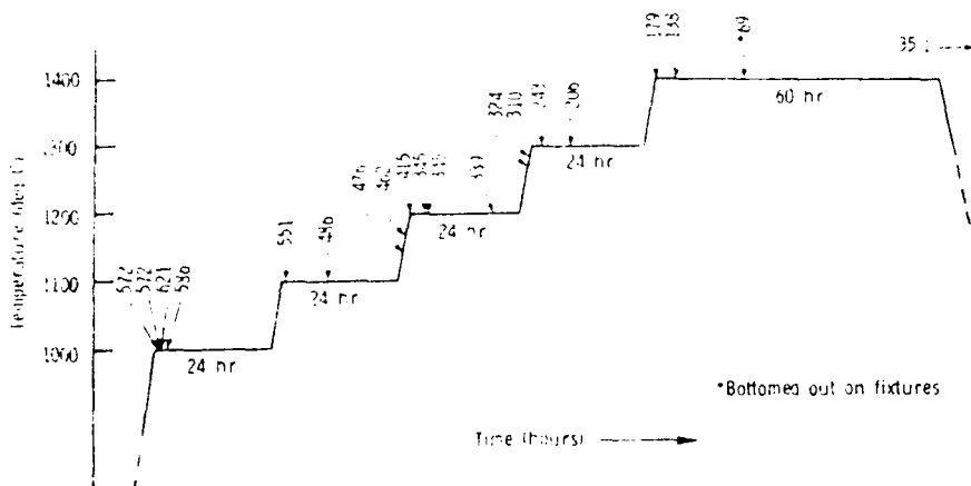
Figure 1. STEPPED TEMPERATURE STRESS RUPTURE DATA FOR NC-132 HPSN. ARROWS INDICATE FAILURE TIMES, ARROW LABELS SPECIFY STRESS ON SAMPLE IN MN/m² (ksi).
