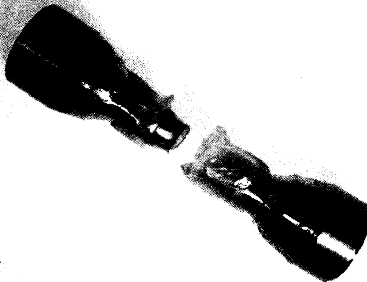
(b) Fractured Specimen After Tensile Testing
