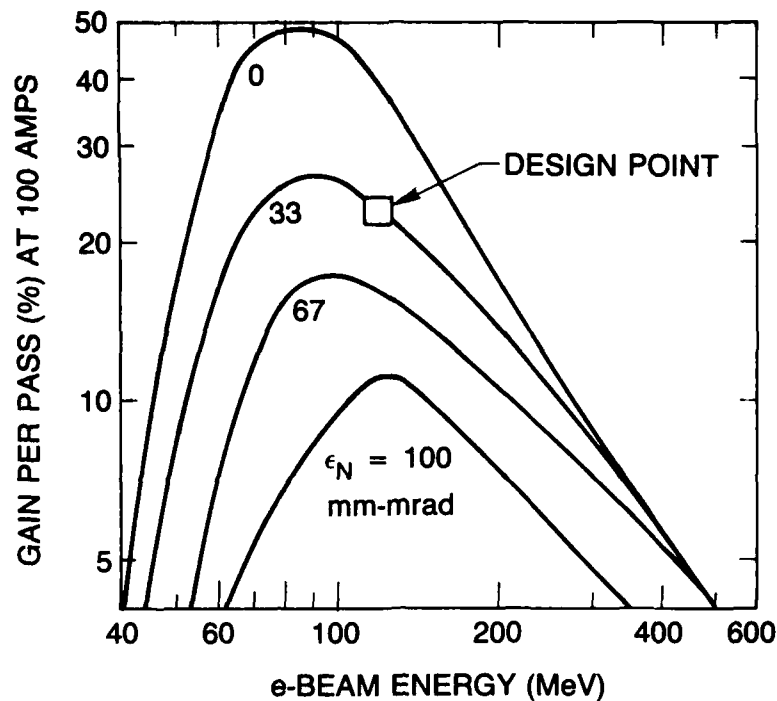
Fig. 7. FEL gain per pass is a sensitive function of linac beam emittance and kinetic energy. These design calculations were based on 0.5- \mu m radiation from a 5-m long wiggler, using 5% extraction and a 100-A micropulse (Ref. 22). Shifting the design point off the peak allows for some uncertainty in the achievable emittance.
