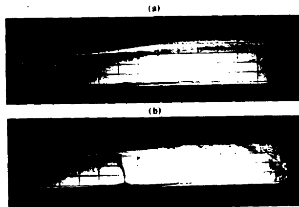
Fig. 5 Spark-Schlieren photographs of attached and separated flow. (a) p_0/p_e = 1.225 (weak shock), (b) p_0/p_e = 1.395 (strong shock). Grid spacing is 24.5-mm horizontally and 12.7-mm vertically.
