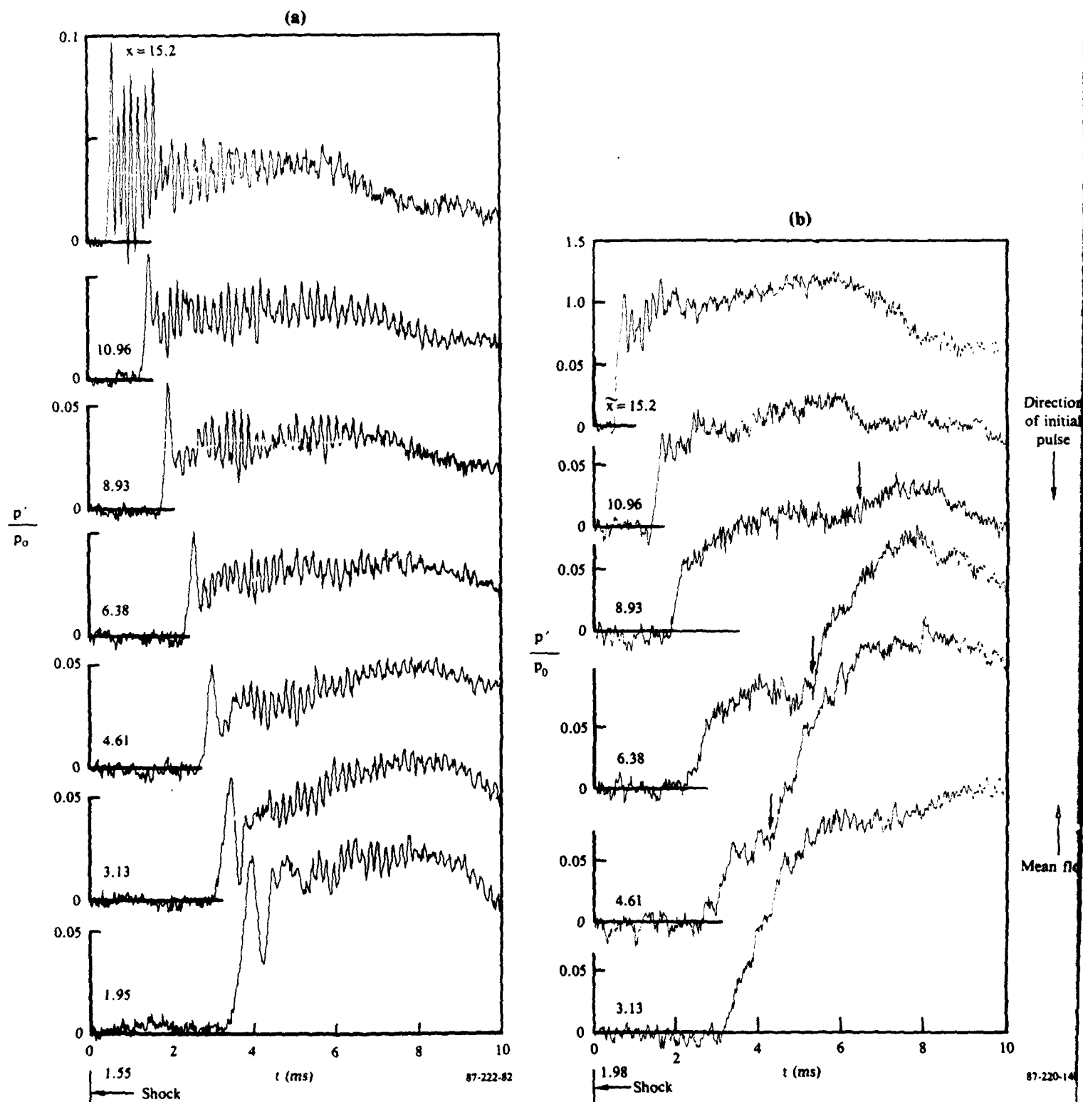
Fig. 10 Time histories of top-wall static pressure: (a) M_O = 1.251 ; (b) M_O = 1.378 . Annotation denotes streamwise transducer location.
