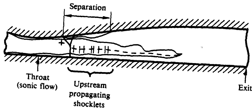
Figure 1. Three basic types of transonic diffuser flows. M_\sigma is Mach number at + signs.
