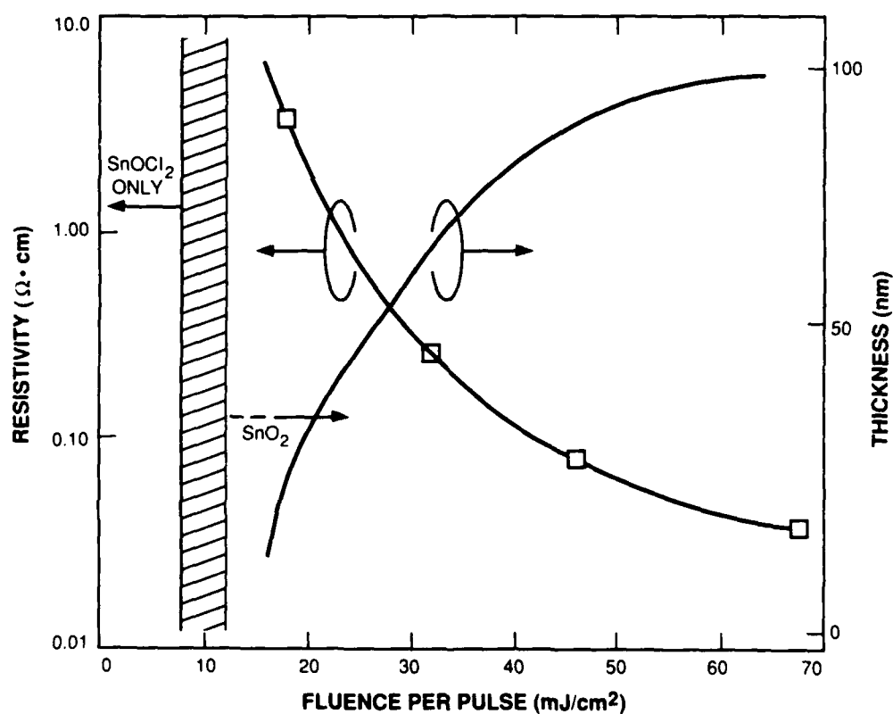
Figure 4-1. Tin oxide film resistivity (left axis) and film thickness (right axis) vs the laser fluence used during growth. For each point, the total number of pulses was fixed at 10^4 , the \text{SnCl}_4 pressure was 0.75 Torr, the \text{N}_2\text{O} pressure 50 Torr, and the laser pulse rate 5 Hz.
