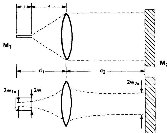
Figure 2-2. Schematic diagram of the external cavity laser. (a) Cross section perpendicular to p-n junction of diode. The active region has length l . (b) Cross section parallel to junction plane. The active region has width 2w .
