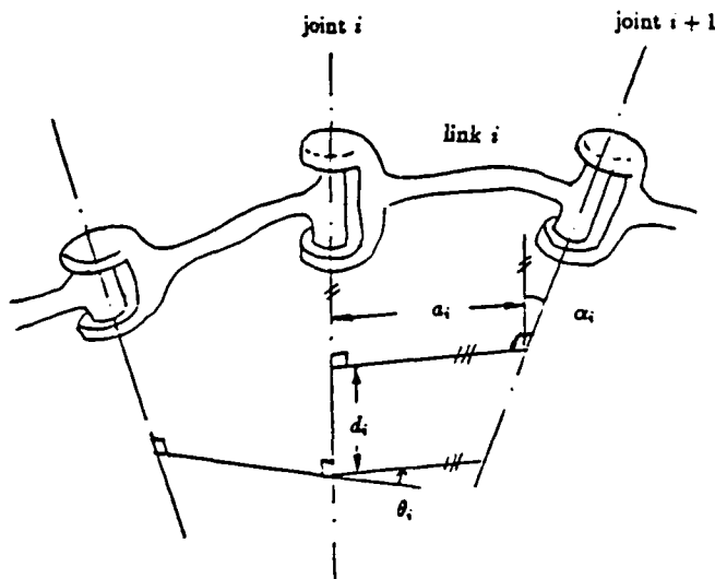
Figure 1: Kinematic parameters of a link
