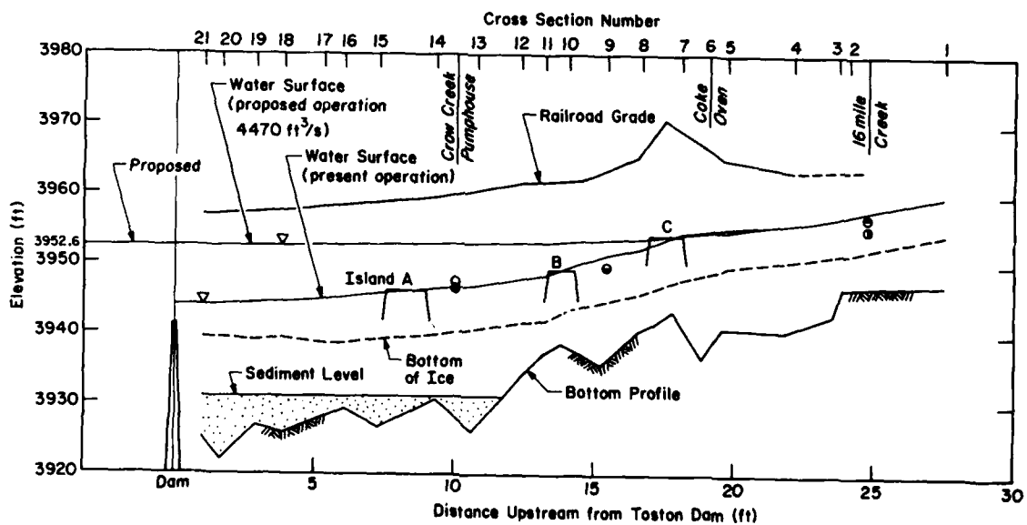
Figure 2. Profiles of water levels and ice thicknesses for discharge of 4470 ft 3 /s under present and proposed dam operating levels.
