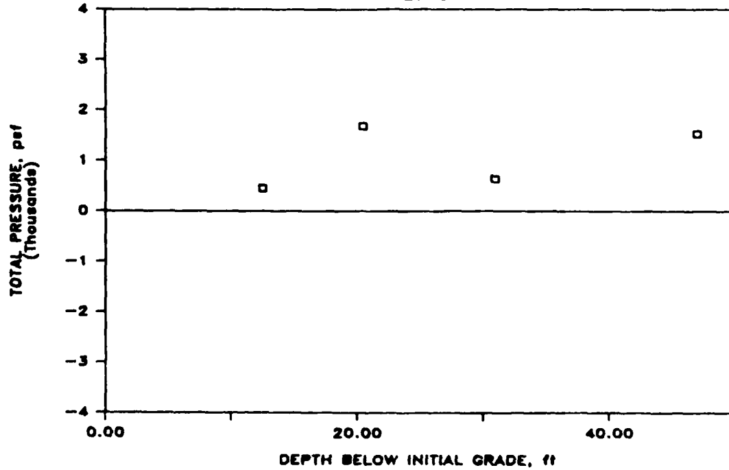
Figure 11. Total pressure distributions for landside wall on 9-19-85 and 1-29-86
