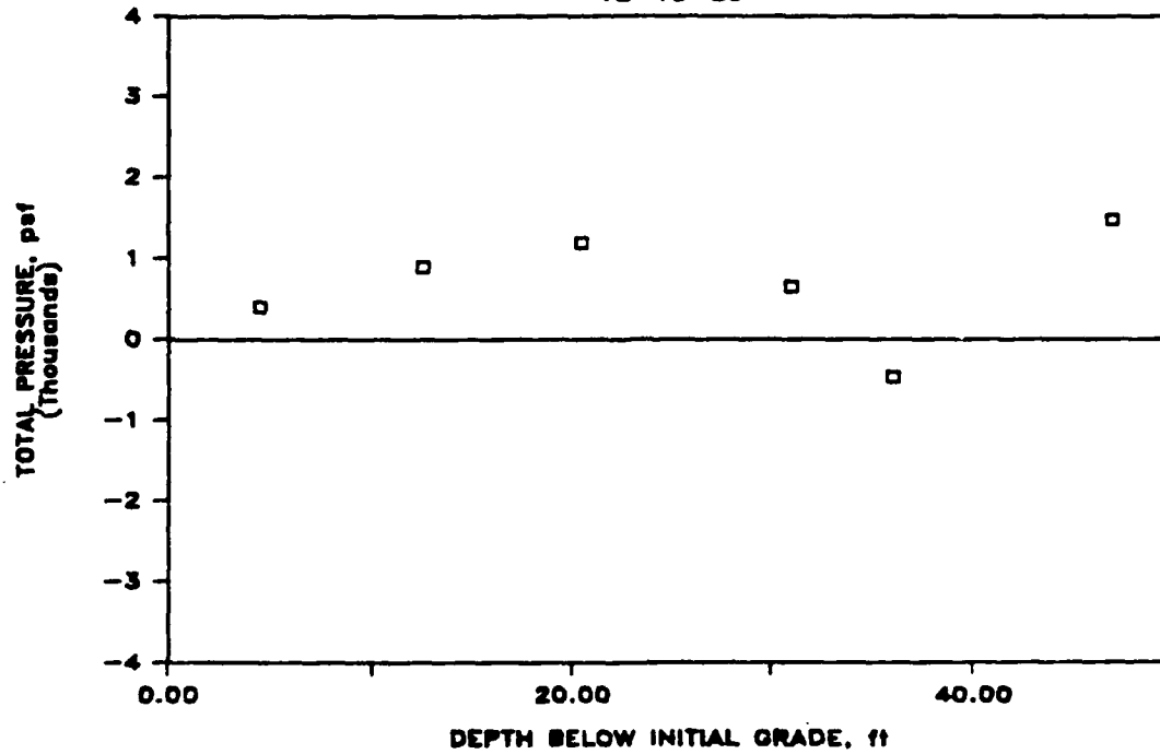
Figure 6. Total pressure distributions for riverside wall on 9-22-83 and 12-13-83
