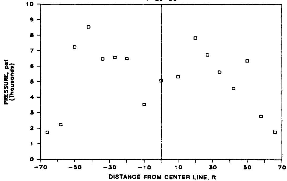
Figure 5. Total pressure distributions for base slab on 9-19-85 and 1-29-86
