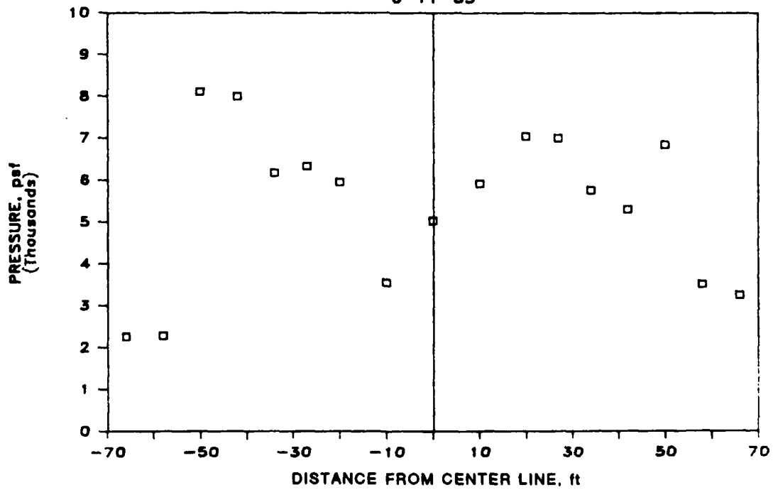
Figure 4. Total pressure distributions for base slab on 3-16-85 and 6-11-85
