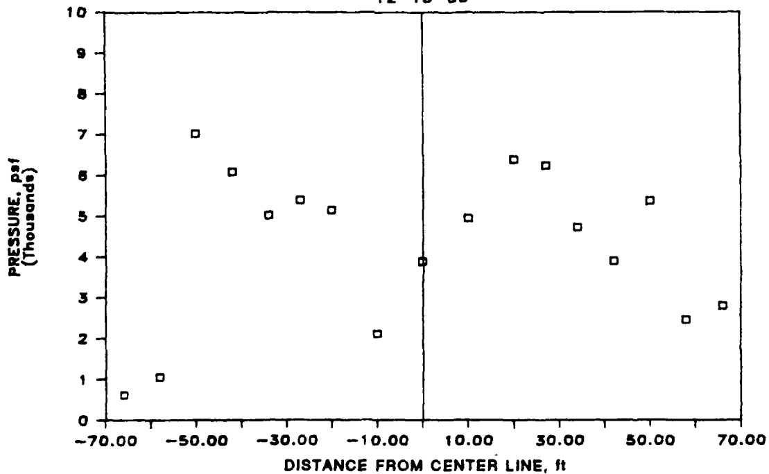
Figure 3. Total pressure distributions for base slab on 9-22-83 and 12-13-83
