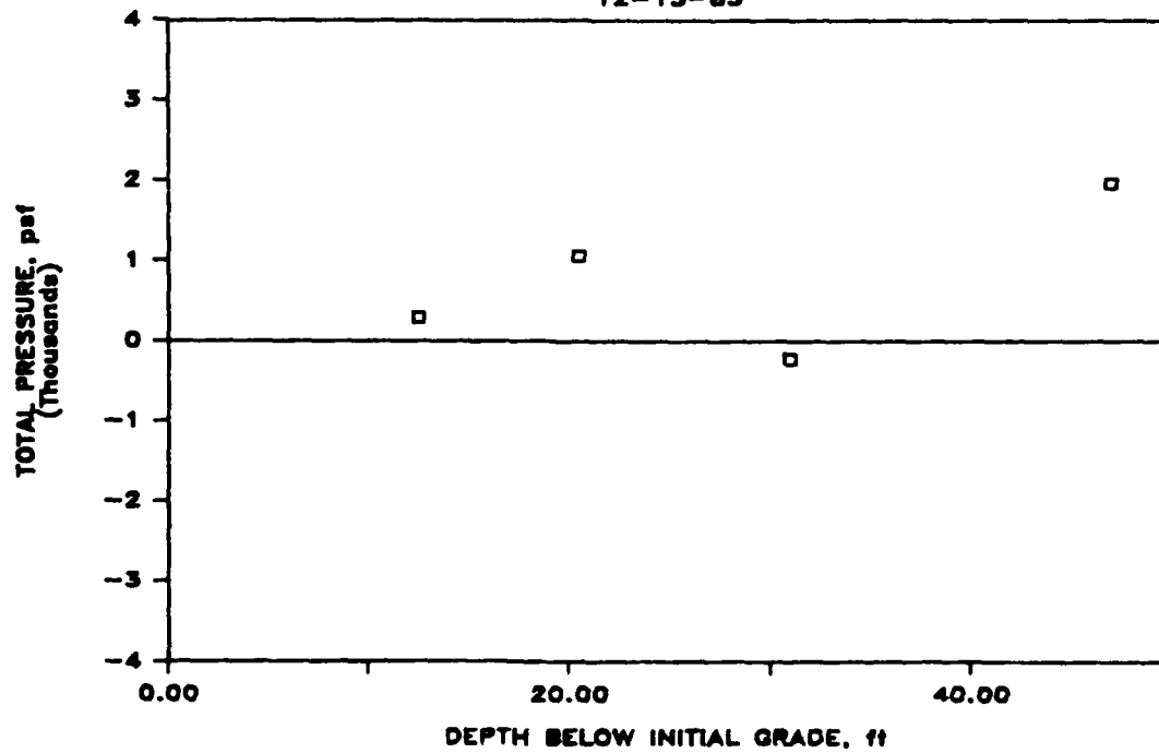
Figure 9. Total pressure distributions for landside wall on 9-22-83 and 12-13-83
