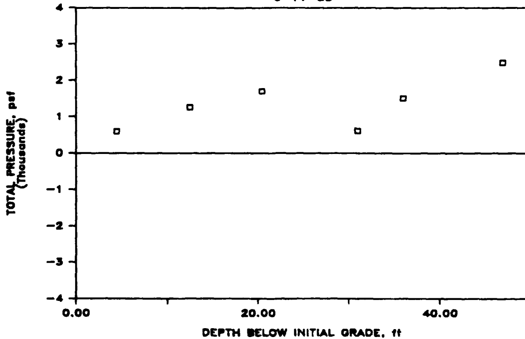
Figure 7. Total pressure distributions for riverside wall on 3-16-85 and 6-11-85
