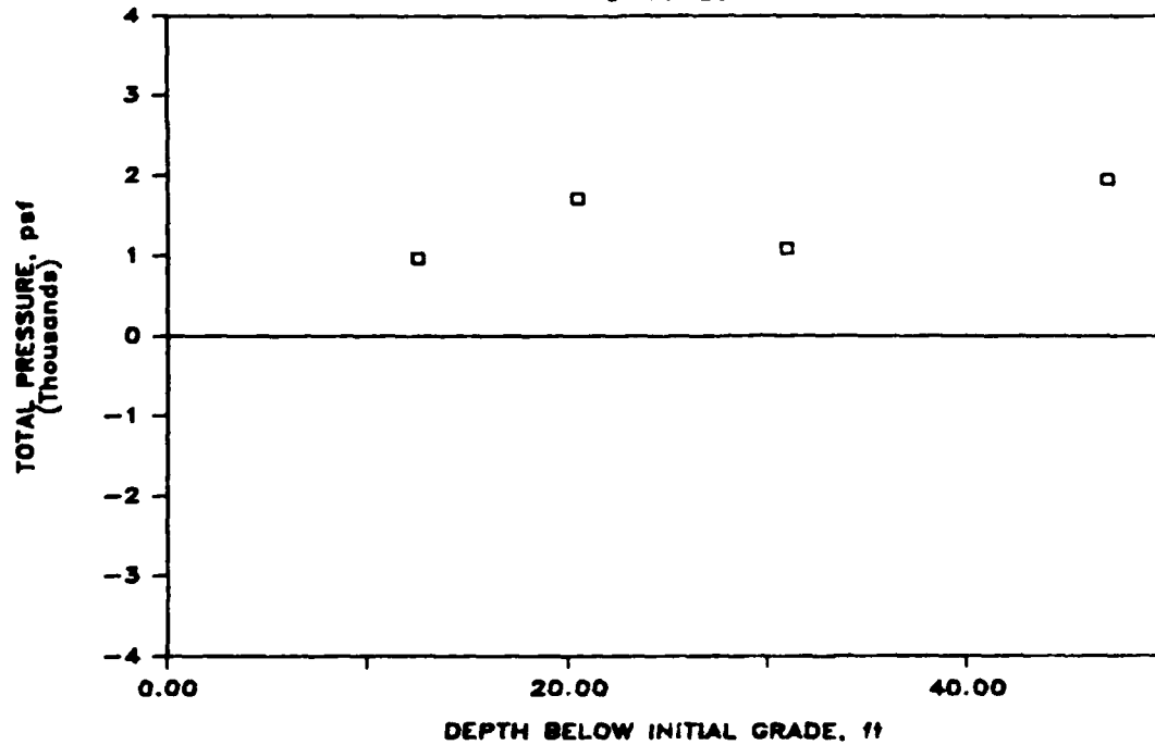
Figure 10. Total pressure distributions for landside wall on 3-16-85 and 6-11-85
