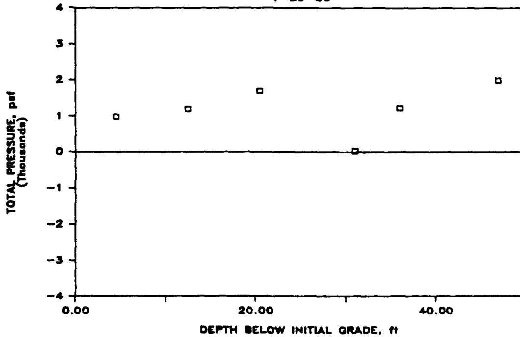
Figure 8. Total pressure distributions for riverside wall on 9-19-85 and 1-29-86
