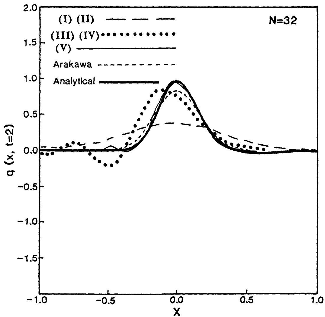
Figure 2. Analytical and numerical solutions with N=32 at t=2 .
