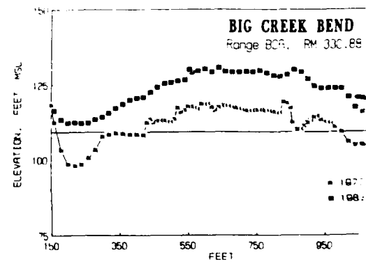
Figure 10. Bendway sedimentation, on cross-section plots is
