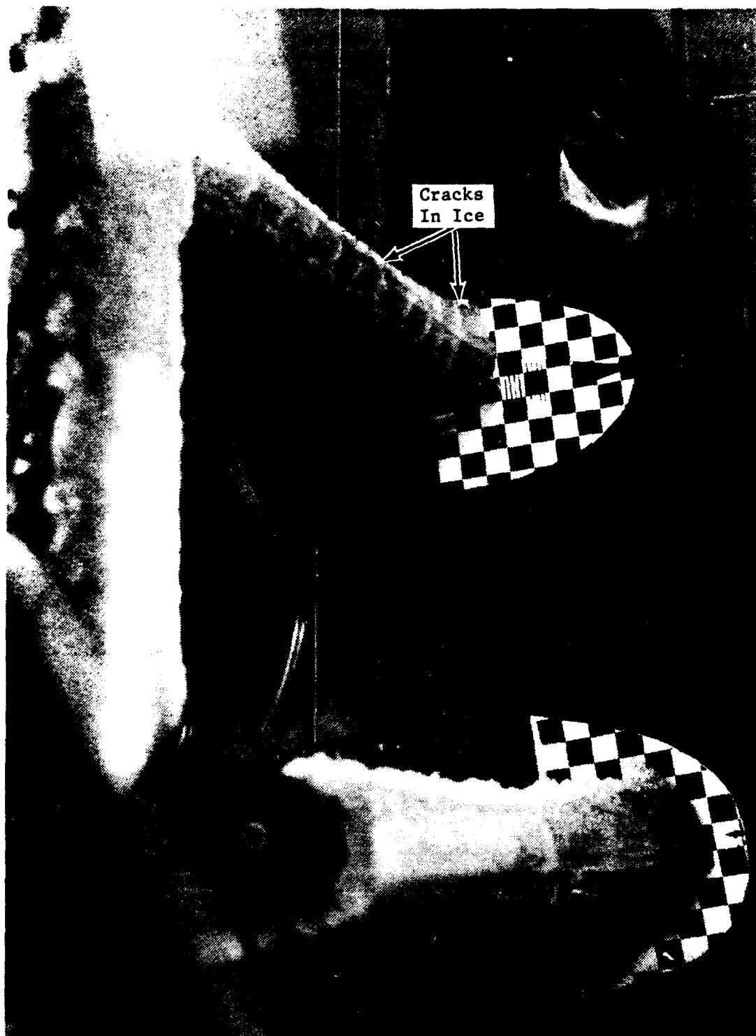
Figure F-18. Vertical Cracks in Ice Accretion Along Span of 6-Inch Chord Airfoil (Top Airfoil)
