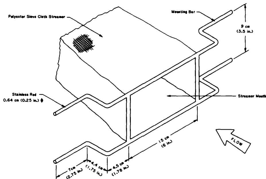
Figure 7. DUCK85 streamer nozzle
