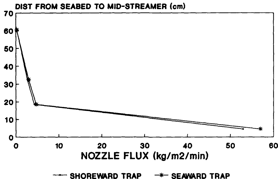
Figure 12. Fluxes measured in consistency Run 85909AM6
