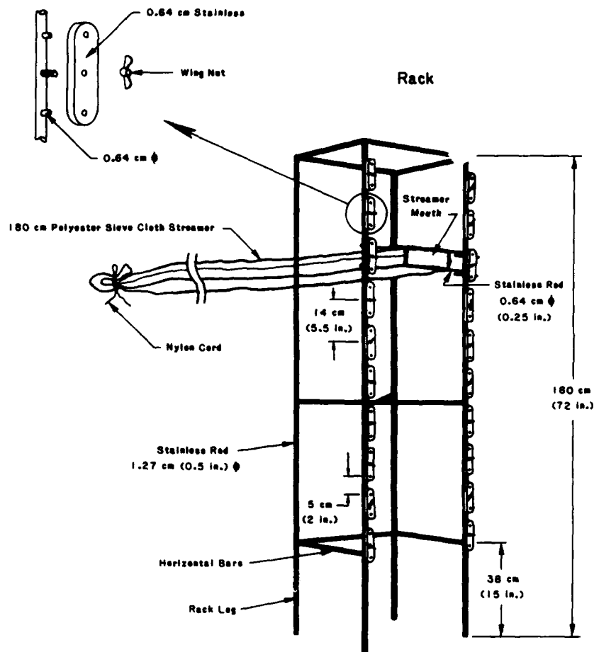
Figure 8. Schematic of the streamer trap rack
