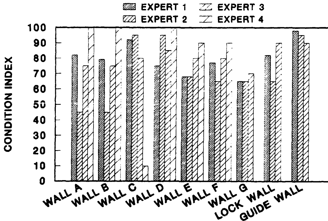
Figure E8. Crack condition index by experts
