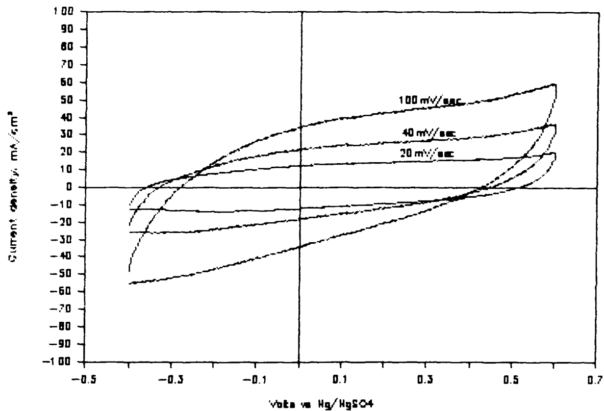
Figure 8a. Voltammograms of \text{RuO}_x Vacuum Impregnated with Nafion and Pressed Against a Nafion Membrane; Tested in Cell of Figure 1.
