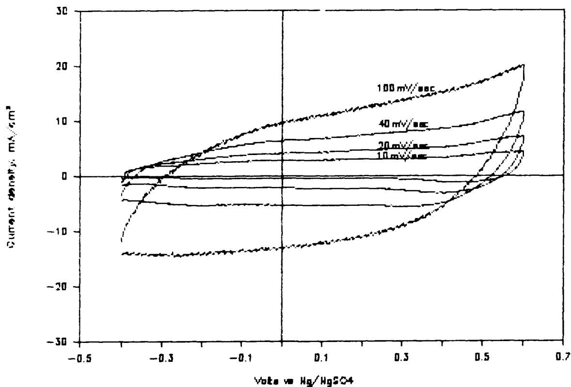
Figure 6a. Voltammograms of \text{RuO}_x Bonded to Nafion Membrane ( 15 \text{ mg/cm}^2 Loading); Tested in Cell of Figure 1.
