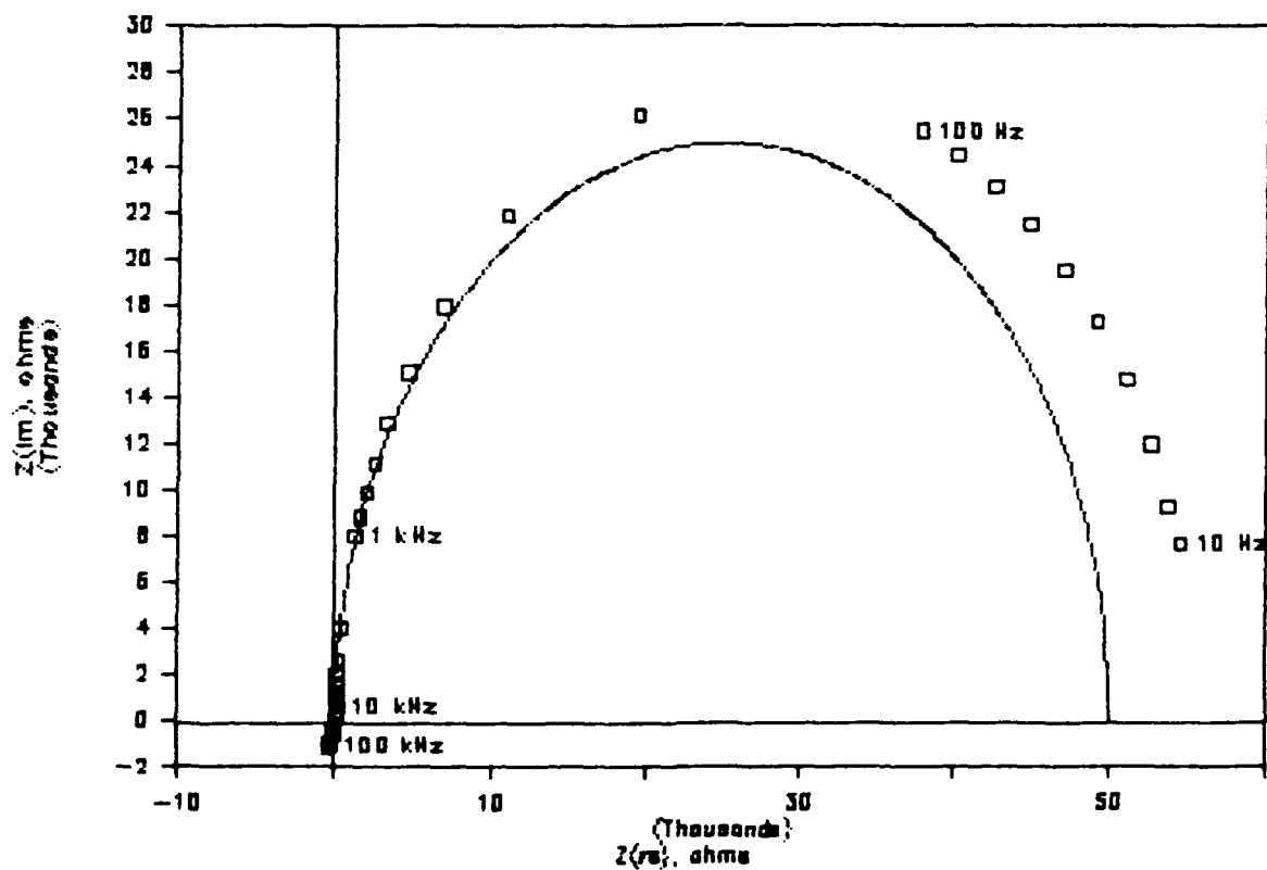
Figure 10. Nyquist Plot for Equivalent Circuit ( 50 \text{ nF} Capacitor in Parallel with 50 \text{ k}\Omega Resistor).
