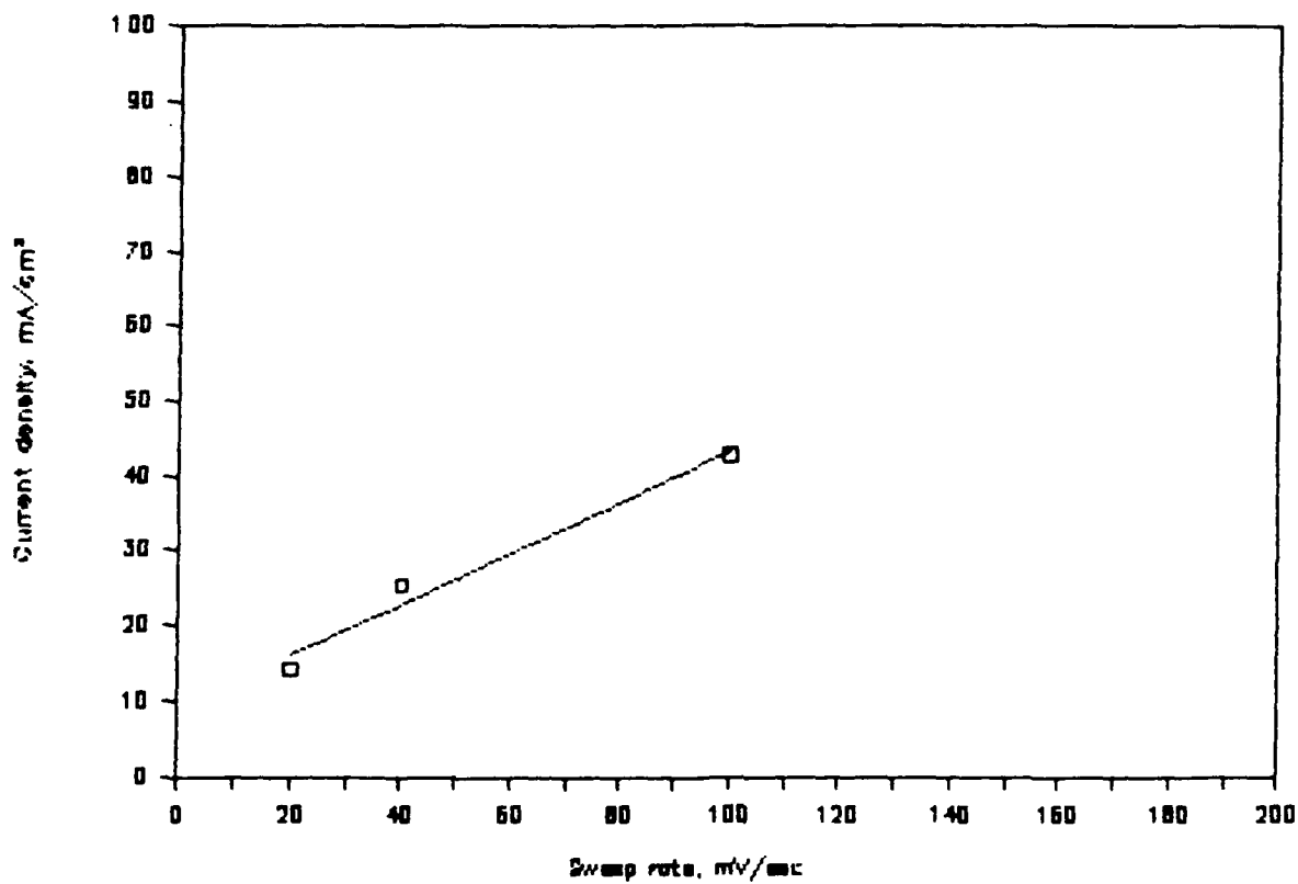
Figure 8b. Current Density vs. Sweep Rate. Calculated Capacitance is 0.342 \text{ F/cm}^2
