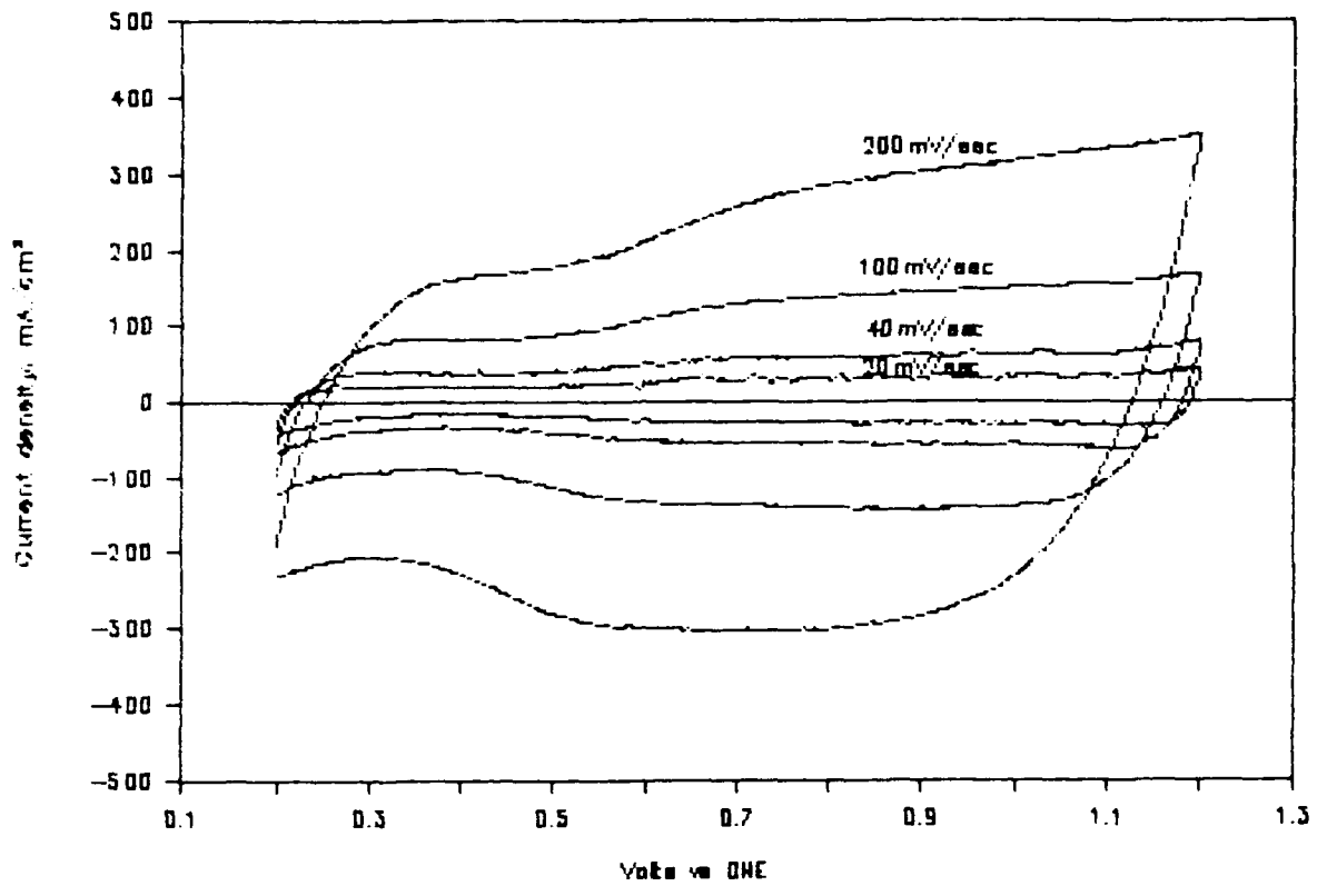
Figure 5a. Voltammograms of \text{RuO}_x Bonded to Nafion Membrane. The outer face of the membrane was in contact with 1M \text{H}_2\text{SO}_4 .
