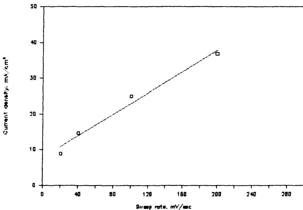
Figure 7b. Current Density vs. Sweep Rate. The Calculated Capacitance is 0.149 F/cm 2 .
