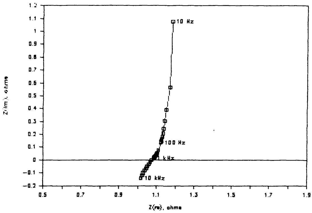
Figure 11. Nyquist Plot for Ferri/Ferro Cyanide Couple.
