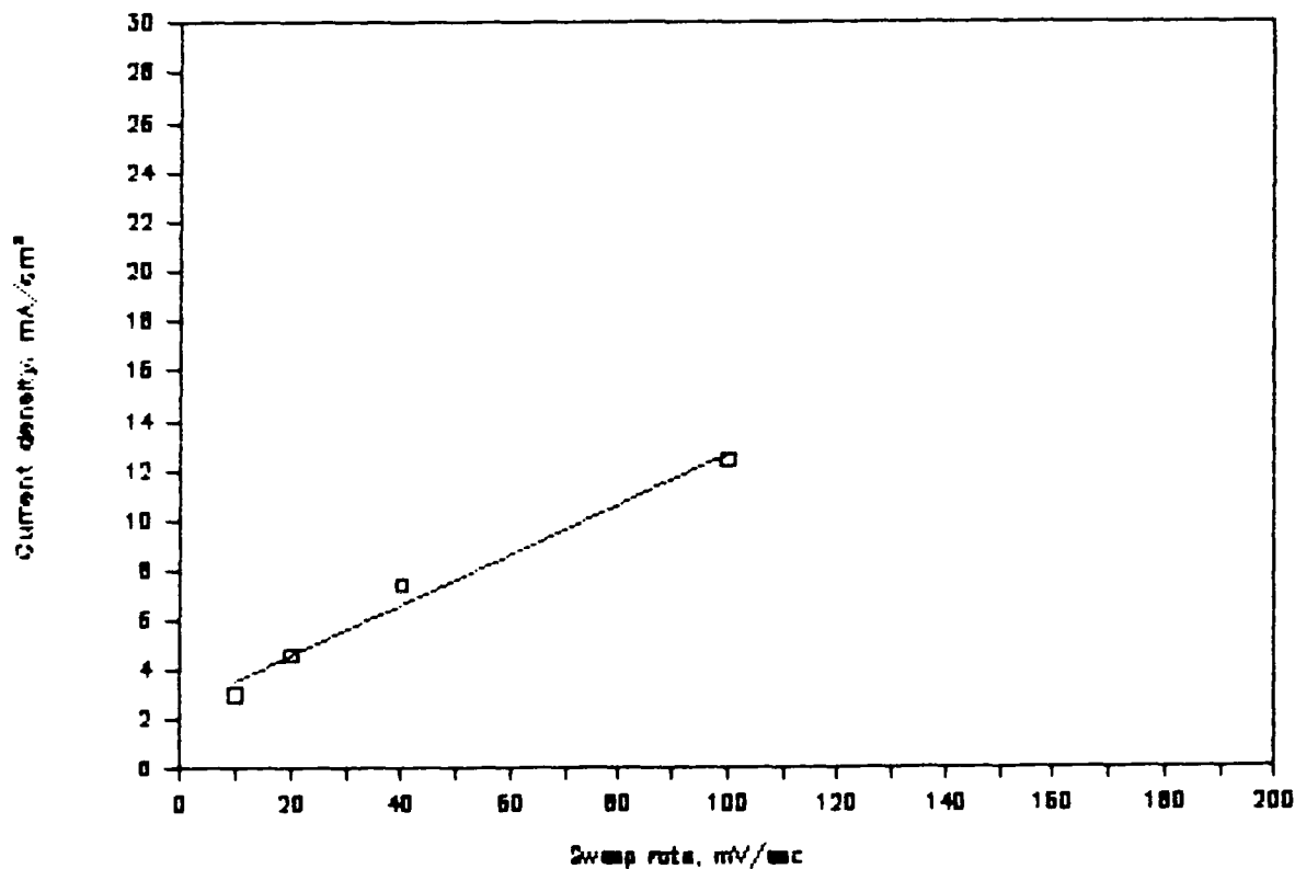
Figure 6b. Current Density vs. Sweep Rate. The Calculated Capacitance is 0.101 \text{ F/cm}^2 .
