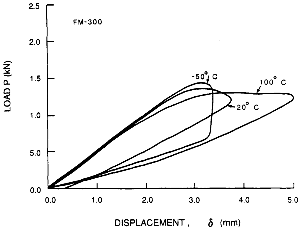
Figure 9. Examples of P- \delta curves for Mode II fracture of FM-300 at different test temperatures.
