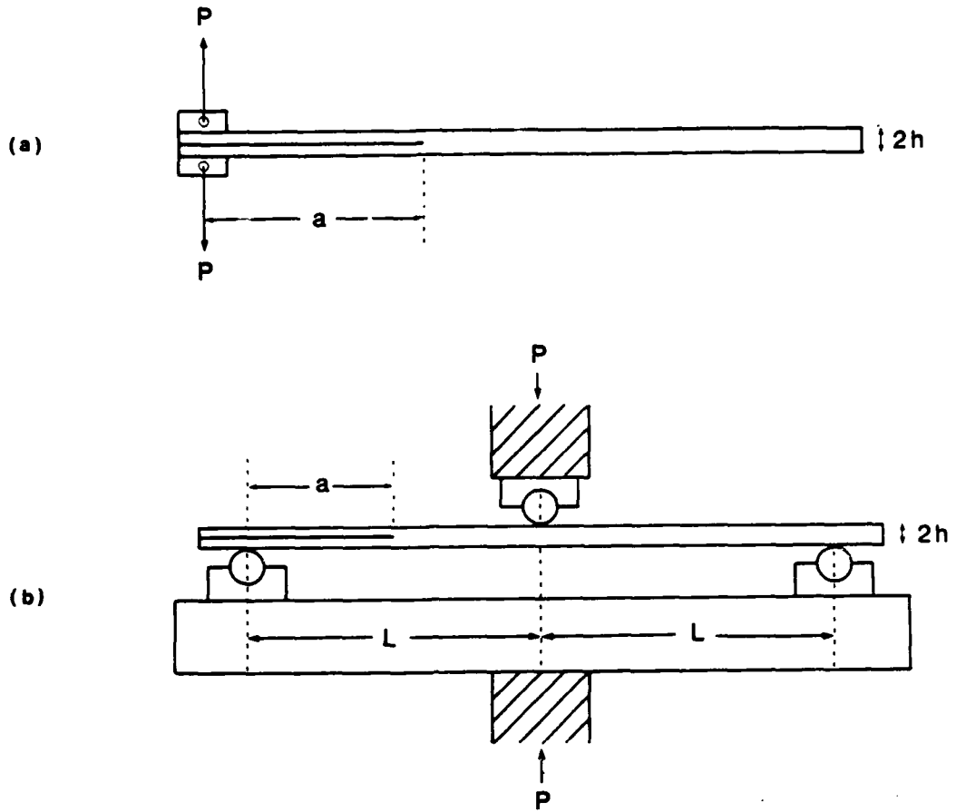
Figure 2. Fracture specimens. (a) Double Cantilever Beam test for Mode I. (b) End Notched Flexure Test for Mode II.
