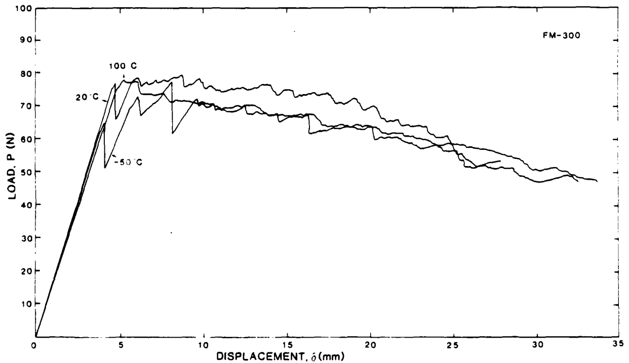
Figure 5. Examples of P- \delta curves for Mode I fracture of FM-300 at different test temperatures.
