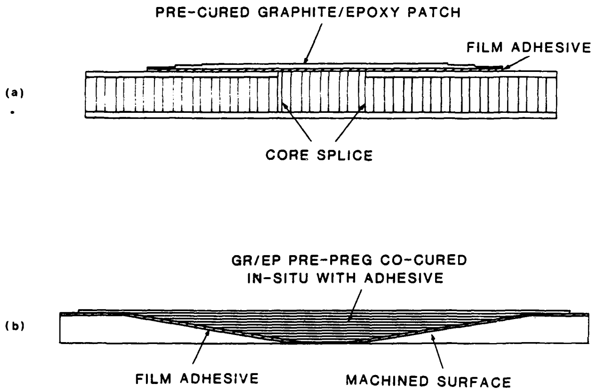
Figure 1. Examples of adhesively bonded repairs. (a) Surface patch bonded to honeycomb sandwich. (b) Scarf repair of monolithic laminate.
