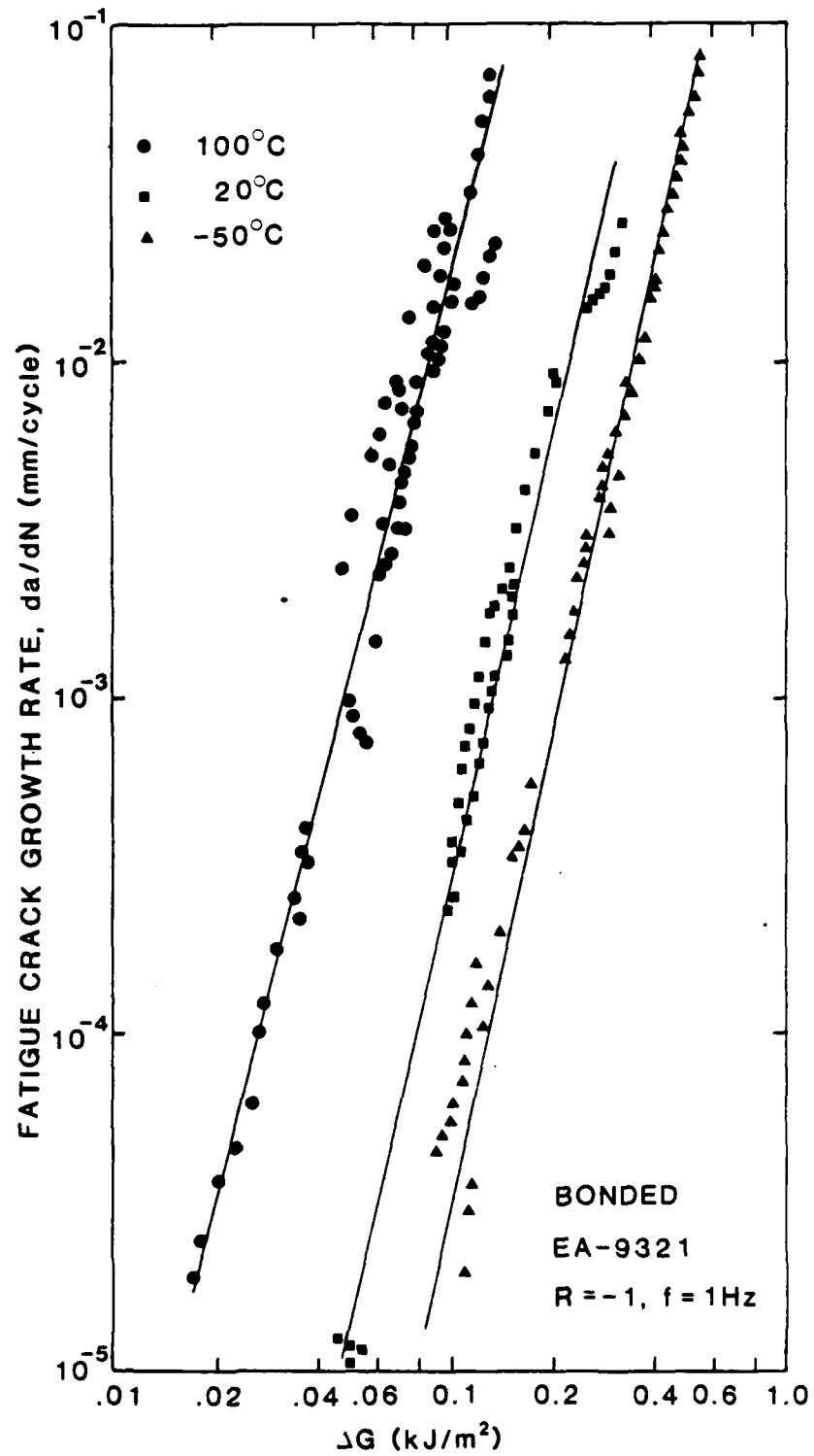
Figure 14. Effect of temperature on the fatigue crack growth rate of EA-9321.
