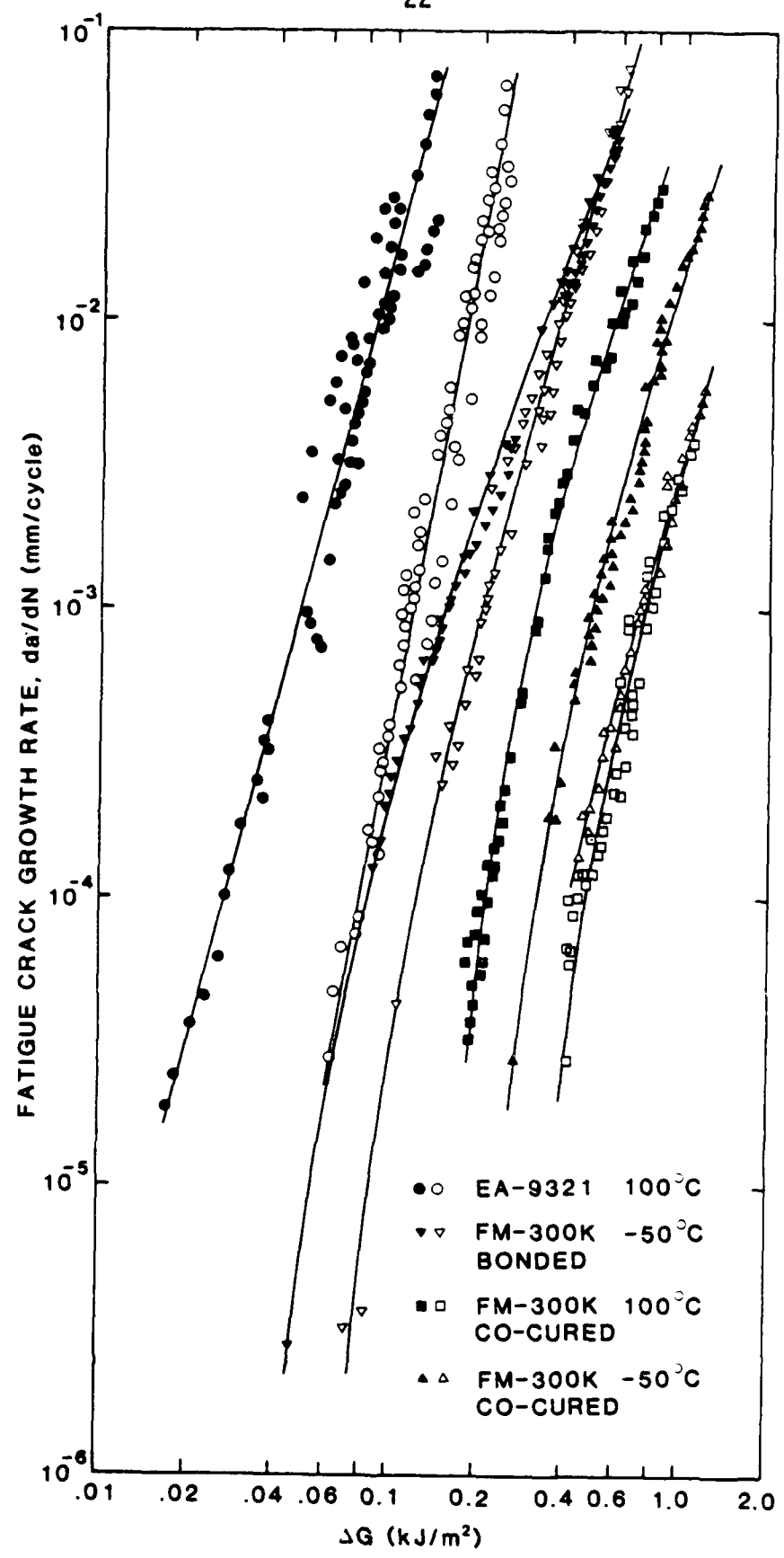
Figure 16. Effect of R-ratio on the fatigue crack growth rate of FM-300K and EA-9321. Open symbols: R=0. Solid symbols: R=-1.
