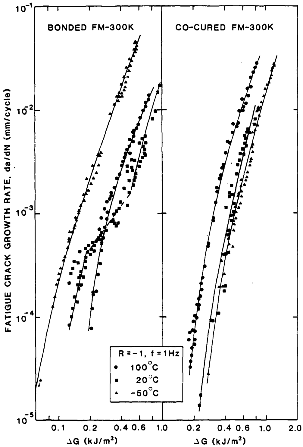
Figure 13. Effect of temperature on the fatigue crack growth rate of FM-300K.
