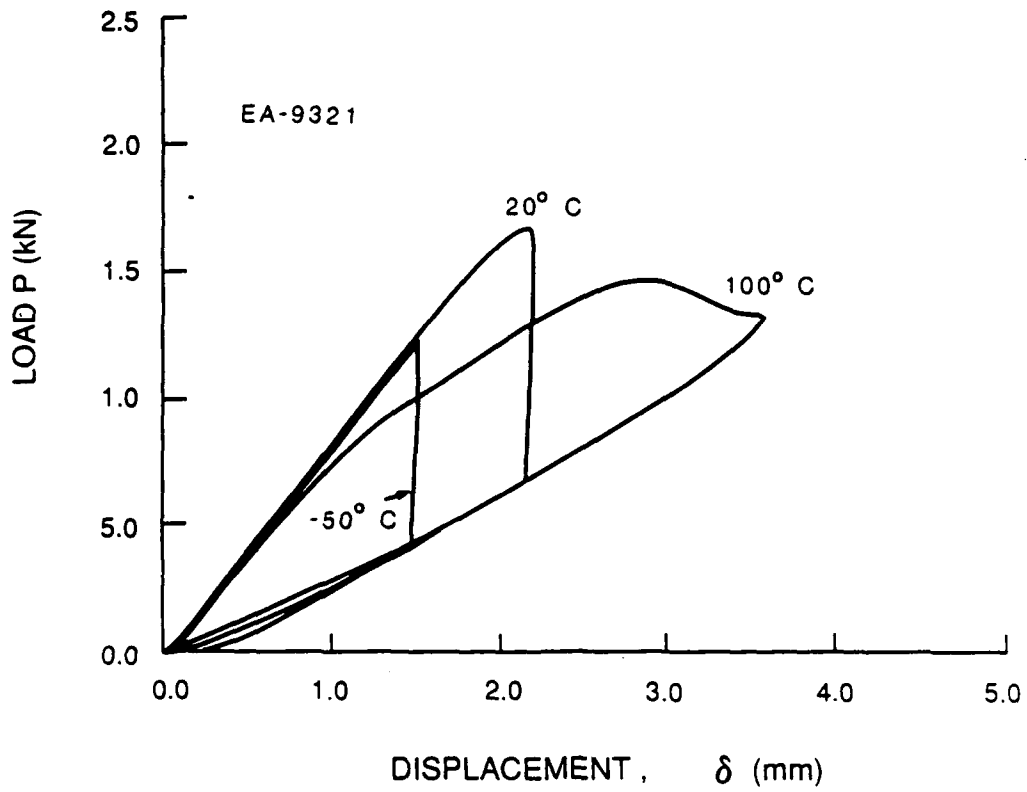
Figure 10. Examples of P- \delta curves for Mode II fracture of EA-9321 at different test temperatures.
