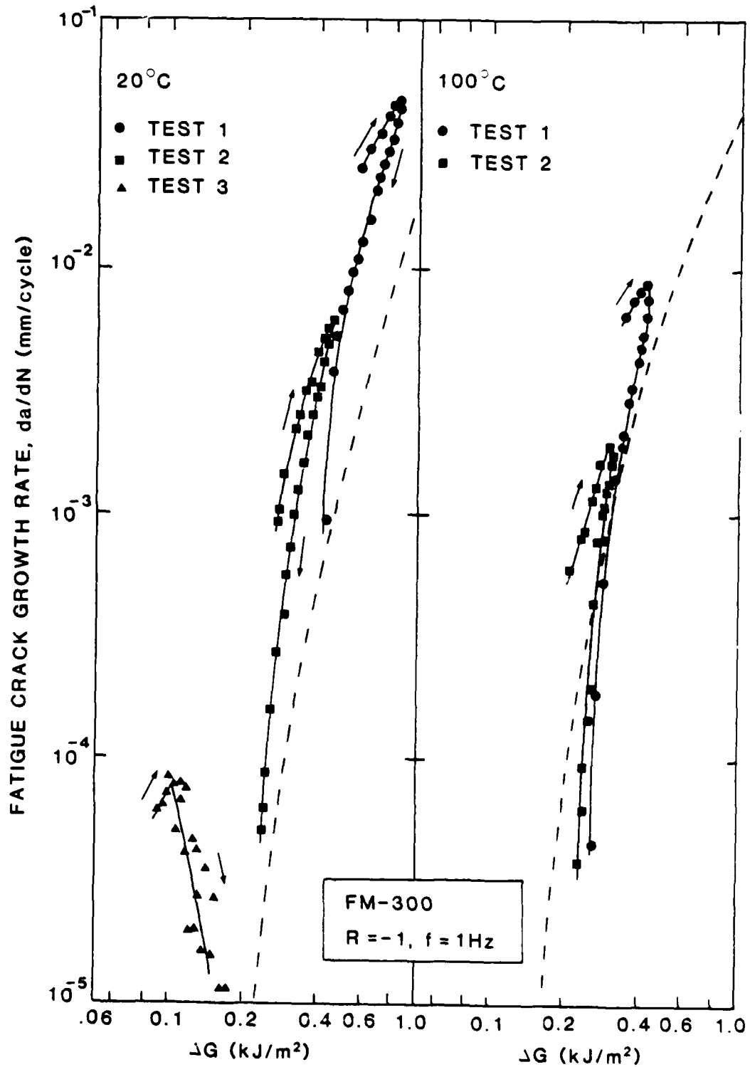
Figure 17. Comparison of fatigue data for co-cured FM-300 at 20^\circ\text{C} and 100^\circ\text{C} with FM-300K curves (dashed lines). Arrows indicate direction of test progression.
