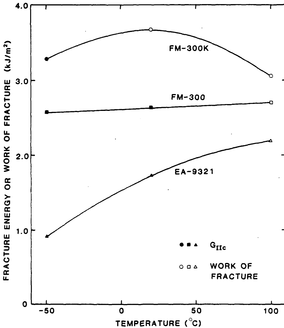
Figure 11. Effect of temperature on the Mode II adhesive fracture energy or work of fracture.
