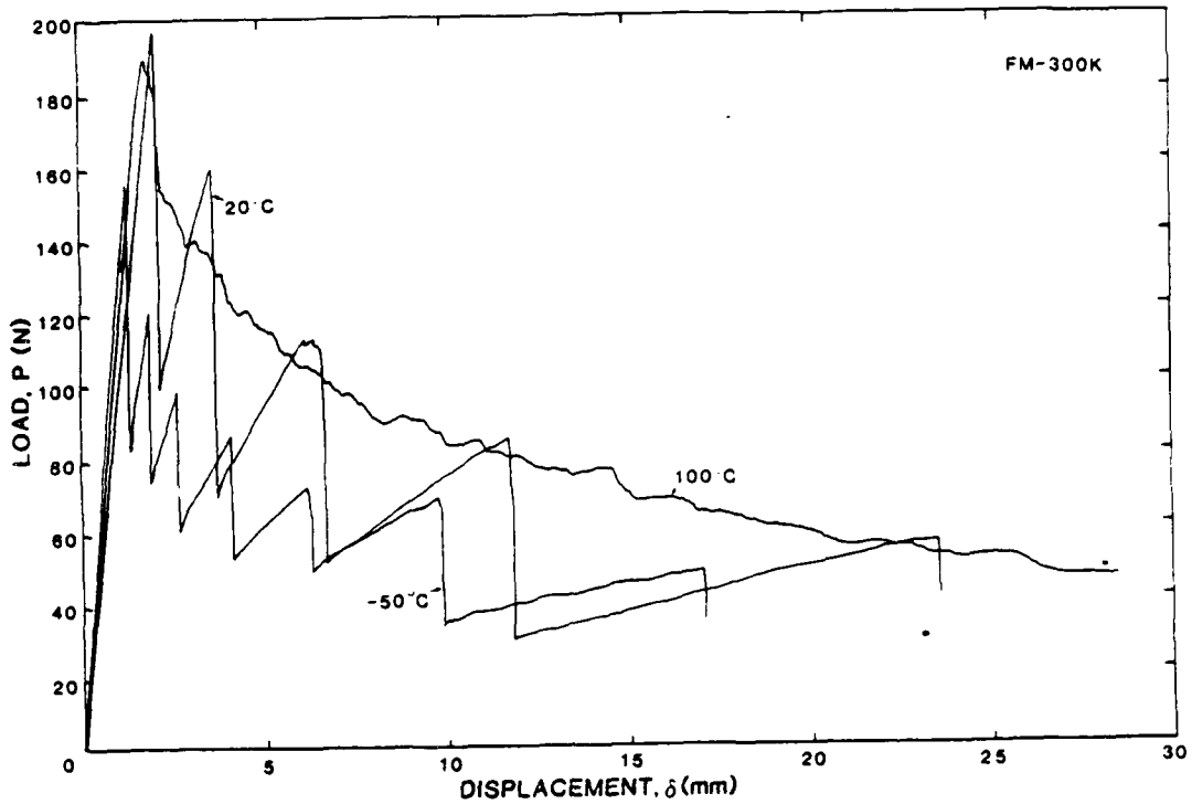
Figure 4. Examples of P- \delta curves for Mode I fracture of FM-300K at different test temperatures.
