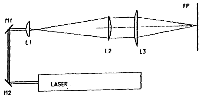
Figure 2 Mounting arrangement
