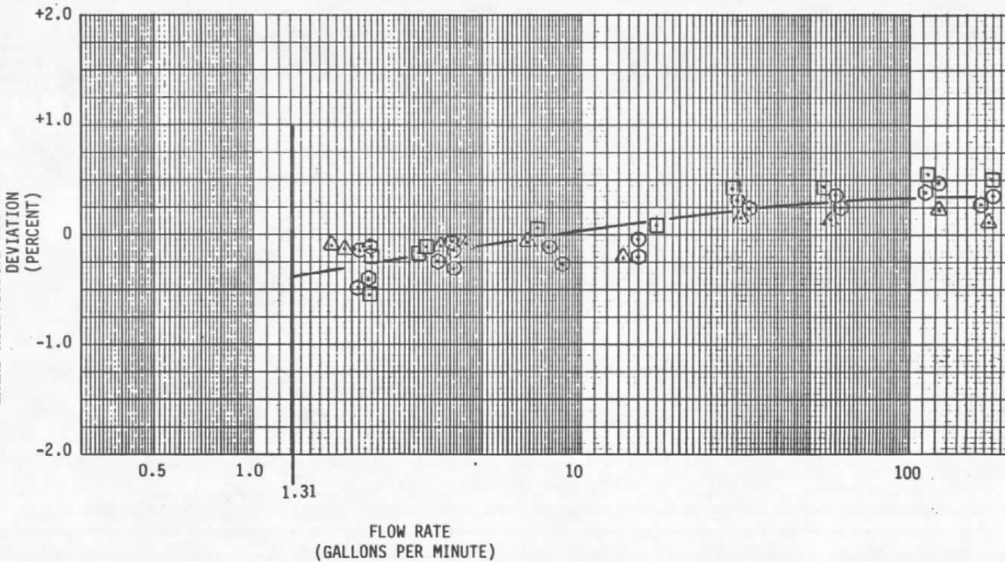
FIGURE 17. COMPOSITE CALIBRATION CURVE
