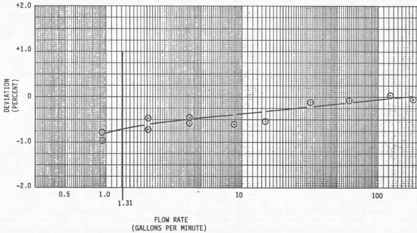
FIGURE 22. STABILITY CALIBRATION NO. 2
