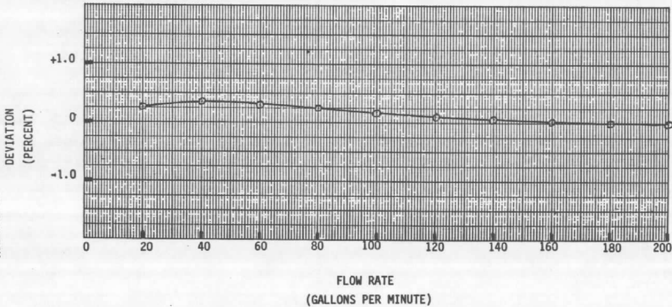
FIGURE 18. MAINSTREAM METER CALIBRATION
