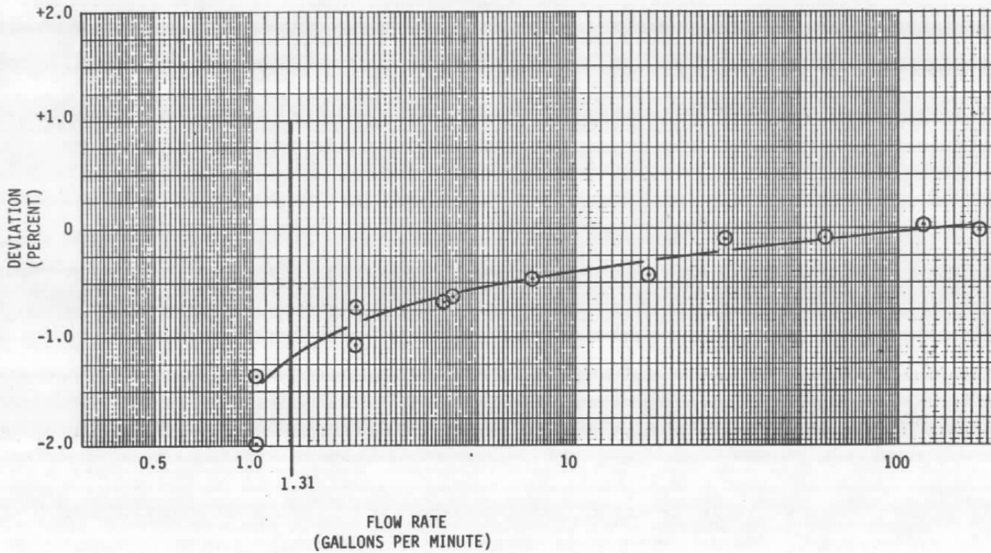
FIGURE 21. STABILITY CALIBRATION NO. 1
