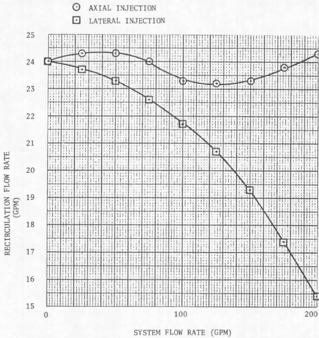
FIGURE 7. CALCULATED RECIRCULATION
