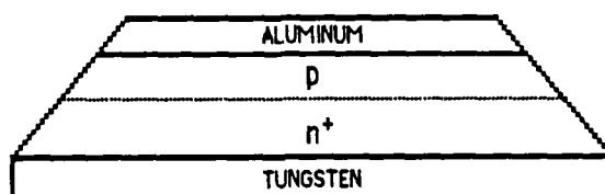
FIGURE 3.3 LASS internal structure
