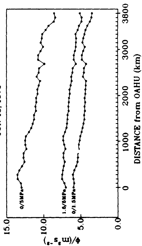
GEOPOTENTIAL ANOMALY JUN 15, 1970
