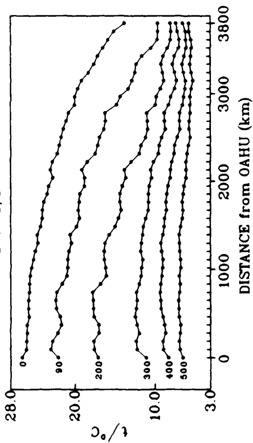
TEMPERATURE at various DEPTHS (meters) SEP 15, 1971
