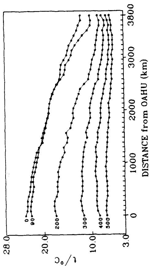
TEMPERATURE at various DEPTHS (meters) JAN 15 MEAN
