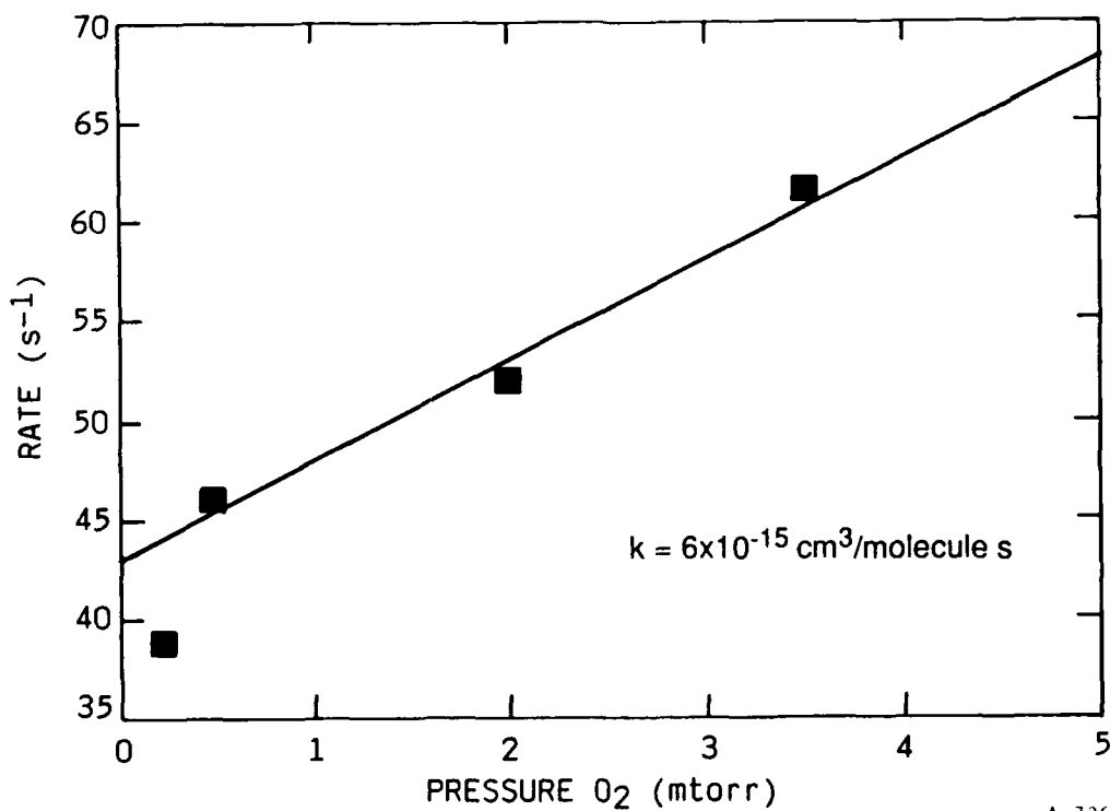
Figure 96. Stern-Volmer plot of O_3^*(v=2) for O_2/Ar mixtures at 30 mtorr Ar.
