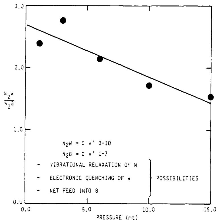
Figure 42. Total quenching of W^3\Delta , v=3-10 state relative to B^3\Pi_g state.
