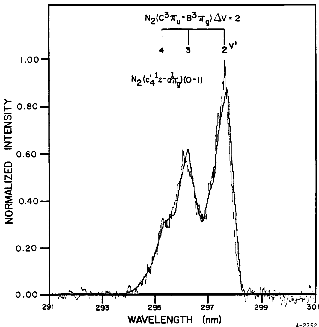
Figure 17. Spectral fit to N_2(C-B) \Delta v=2 sequence band with (c'_4-a) 0-1 band included.
