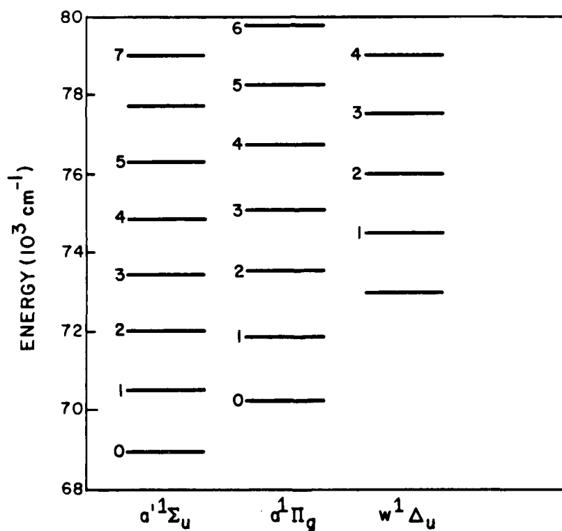
Figure 13. Energy level diagram for N_2 singlets.
