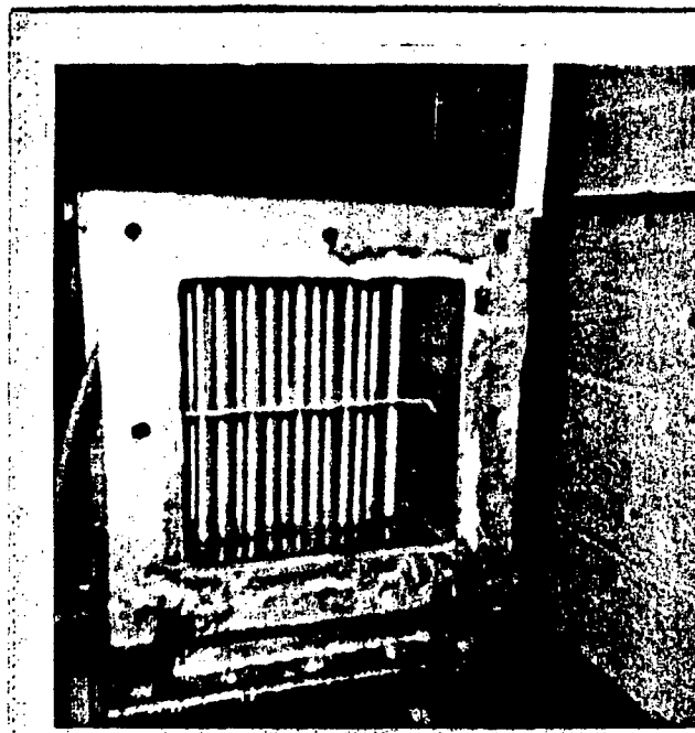
Figure 5-6: Photos of the Experimental Rig and the Model Heat Pipe Heat Exchanger
