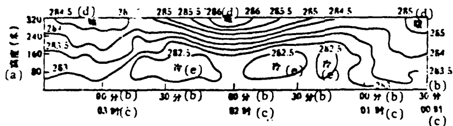
Fig. 2. Time-space distribution of \theta values from 0030 to 0330 hours on 27 August 1980. Key: (a) Altitude (meters); (b) Minutes; (c) Hours; (d) Warm; (e) Cold.
