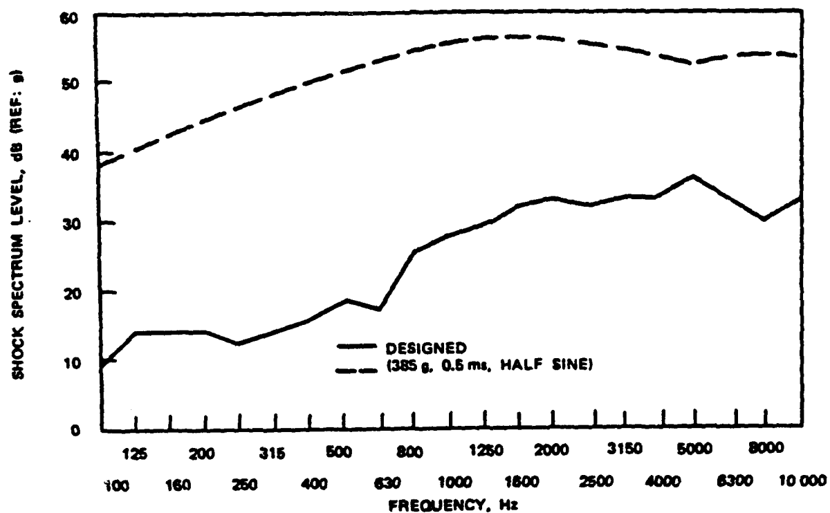
Figure 5-40(a) Comparison of Q = 10 Shock Spectrum Levels and Design Criterion for the Midcourse Guidance Unit (Reference 21)
