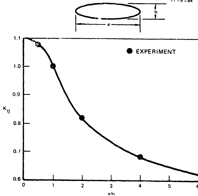
FIGURE 34 CORRECTION OF VISCOUS CROSS-FLOW FOR ELLIPTICAL CROSS-SECTIONS IN SUBCRITICAL FLOW
