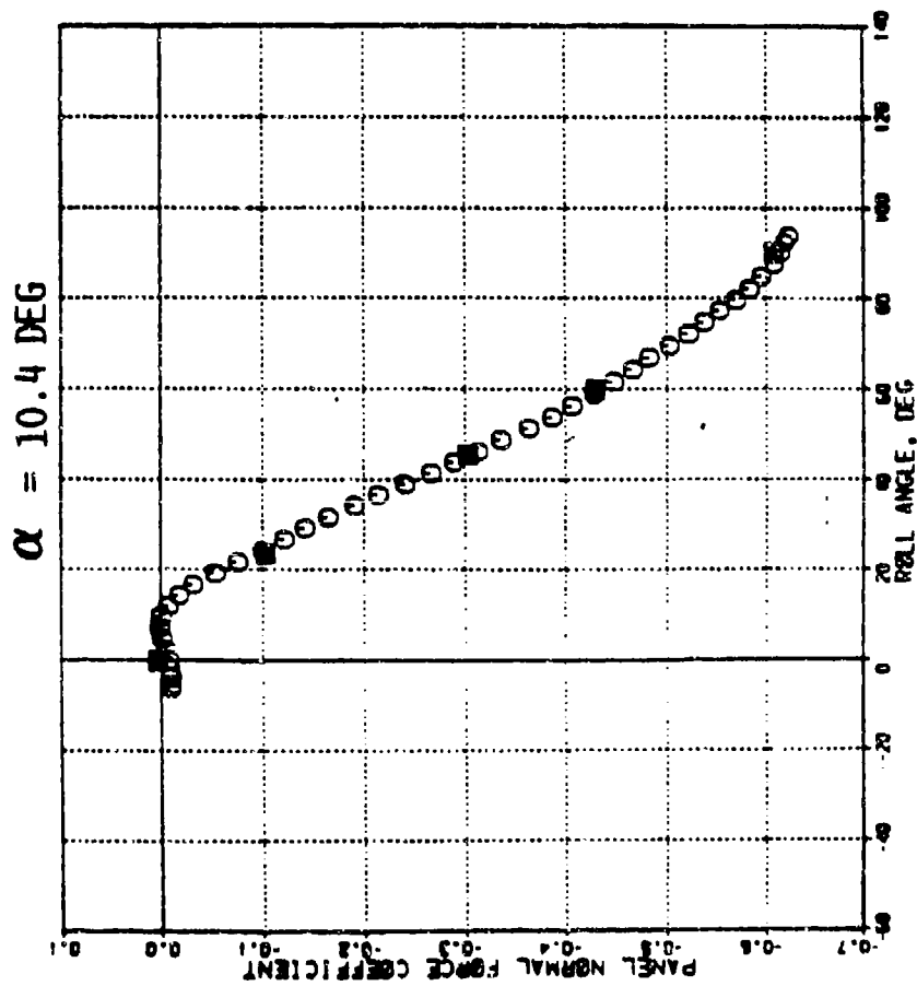
FIGURE 57 TRANSONIC PANEL LOAD PREDICTIONS GOOD
