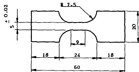
FATIGUE SPECIMEN K_t=1
