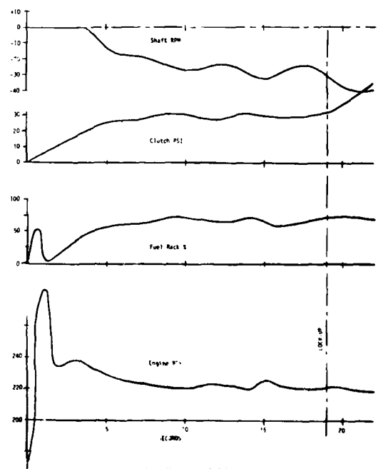
Figure 6 Simulated Clutch-In Shaft Released
