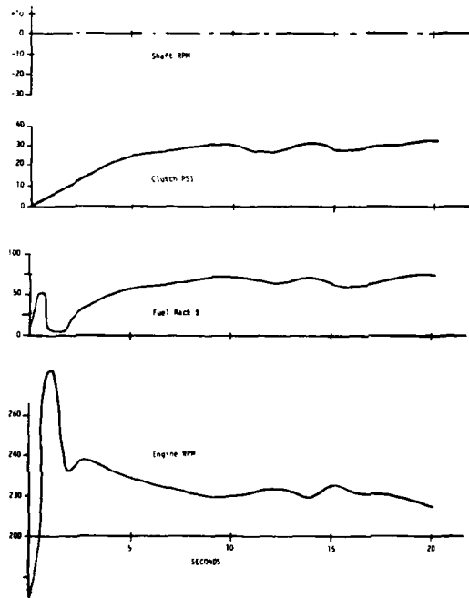
Figure 5 Simulated Clutch-In with Shaft Locked
