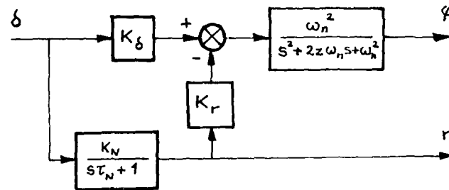
Figure 4 Simplified block diagram
