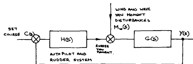
Figure 7. Autopilot System
