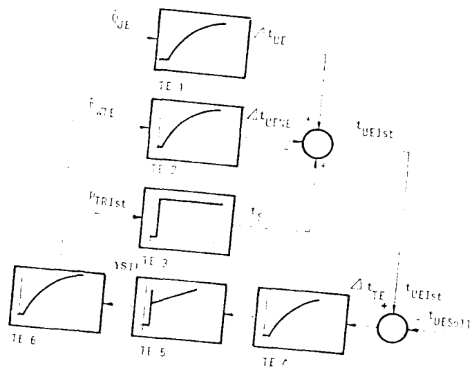
Figure 1. Superheater temperature control cycle
