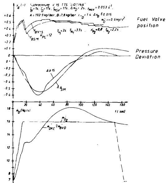
Figure 25. Comparison Shipboard Test with Simulation
