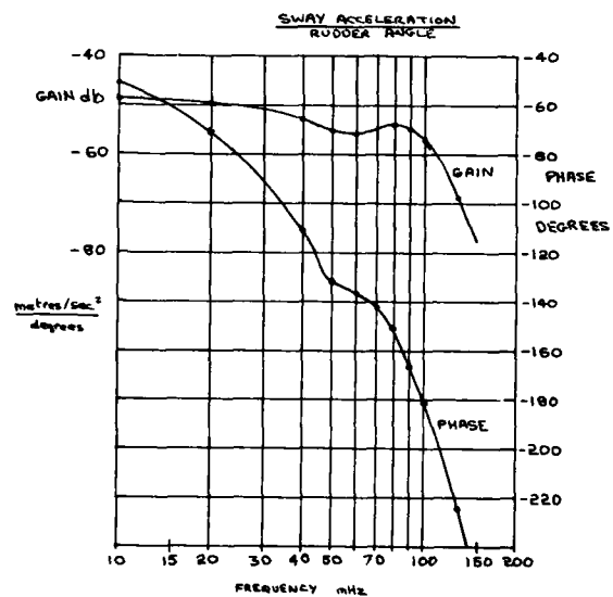
Figure 21. Frigate 16 Knots Rudder Angle to Sway Acceleration F2 2-22
