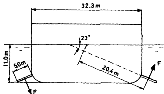
Figure 1. Active Pins Designed for the Test Ship.
