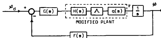
Fig(7): Two degree-of-freedom yaw control system for simultaneous satisfaction of sensitivity and response specifications.
