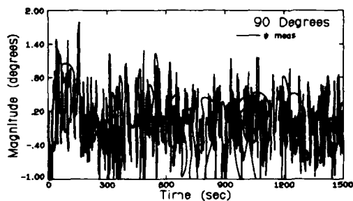
Figure 24 Yaw Measurement at 90 Degree Encounter Angle: 250,000 DWT Tanker, Beaufort 8, 15 Knots, Controller L11 with Measurement Noise
