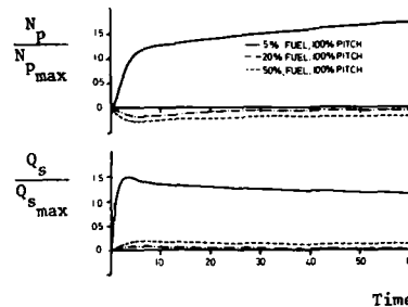
Figure 3. Response of Open-Loop System to Step Input on Pitch.
