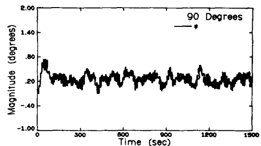
Figure 25 Yaw at 90 Degree Encounter Angle: 250,000 DWT Tanker, Beaufort 8, 15 Knots, Controller L11 with Measurement Noise
