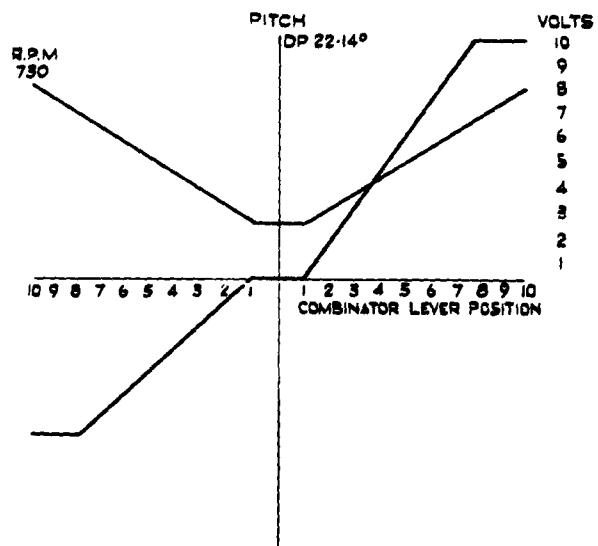
Figure 8. Combinator Diagram.
