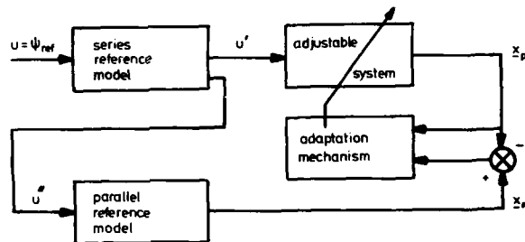
Figure 3 : Simplified block diagram of MRAS in course changing mode
