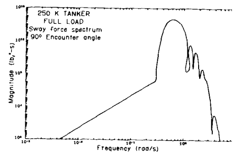
Figure 12 Sway Force Spectrum, 90 Degree Encounter Angle: 250,000 DWT Tanker Full Load, Beaufort 8 Conditions
