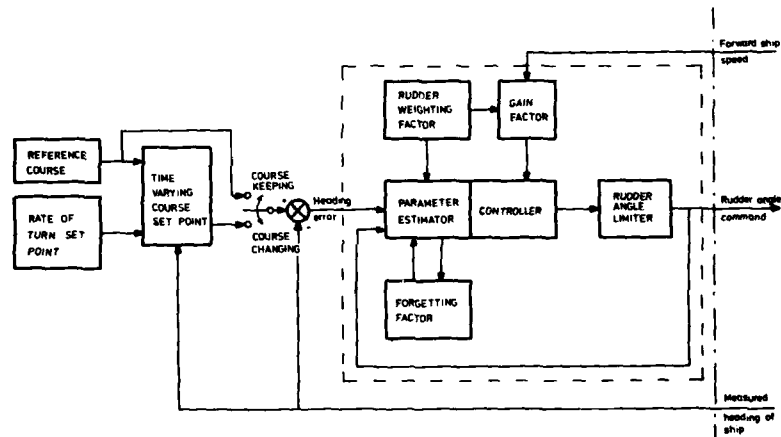
Figure 5 : Simplified blockdiagram of STR - autopilot
