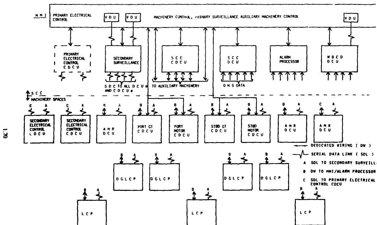
Figure 5 System Configuration
