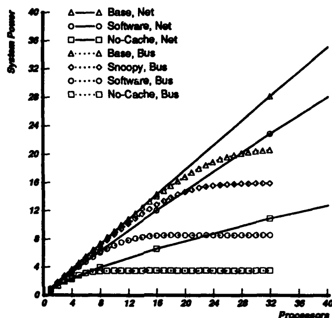
Figure 10: Buses versus networks in the small scale.
