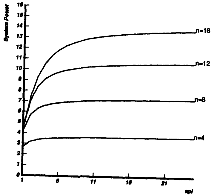
Figure 8: Effect of apl with low sharing; other parameters at medium values
