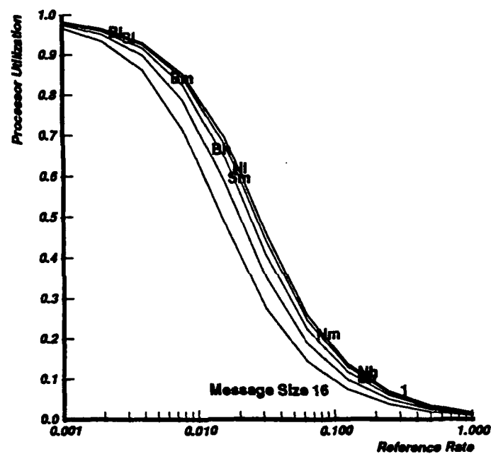
Figure 11: Bus performance for various request rates and with message sizes of 1, 2, 4, 8 and 16 words. The performance of the Base, Software-Flush, and No-Cache schemes is marked with two letter codes, the first letter (B, S, or N) corresponds to the scheme, and the second letter corresponds to a low, middle, or high (l, m, or h) range.
