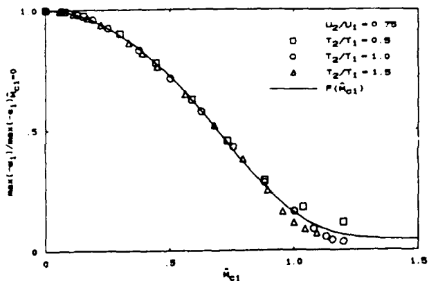
Figs. 4-9 Normalized maximum amplification rate vs M_{C1} .
