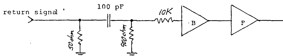
Figure 15. Improved "leading edge" circuit
