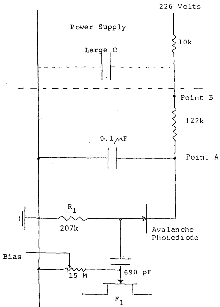
Figure 2. Circuit for gain regulation on the Avalanche Photodiode.
