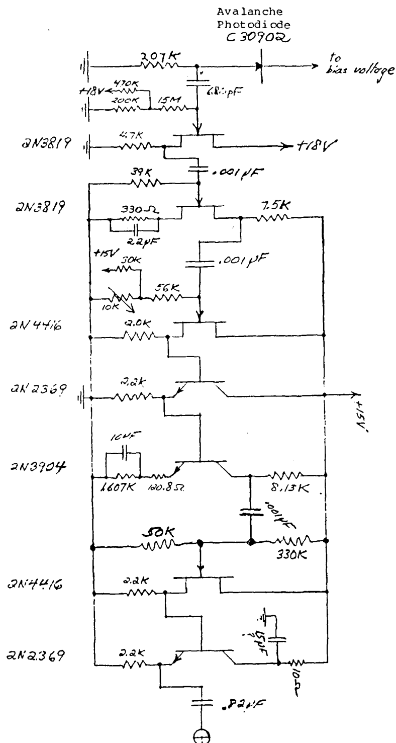
Figure 1. Pulse amplifier circuit
