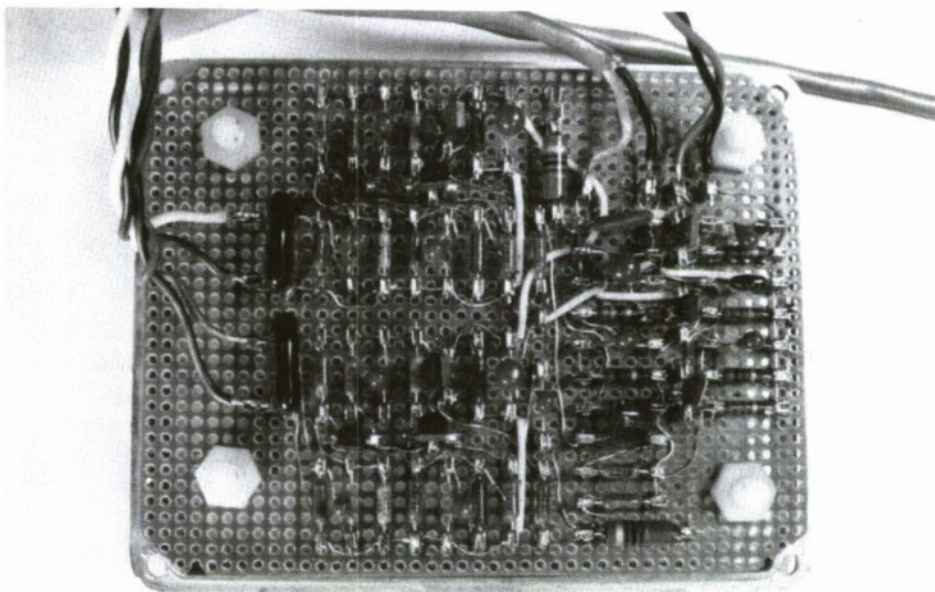
Figure 4b. The Active Component Housing
