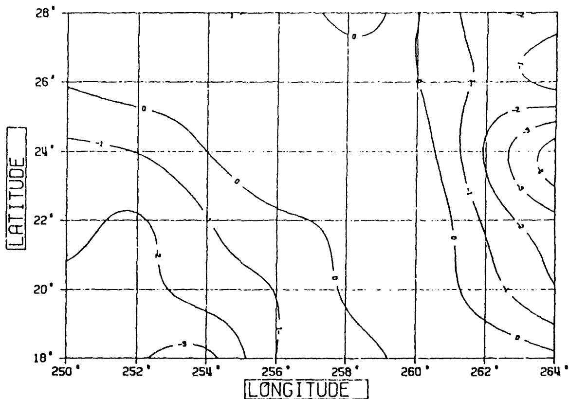
Figure 2.4: Contours of the line of sight acceleration to the third GPS satellite.
