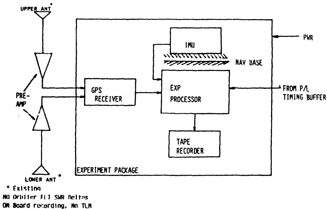
FIGURE 6.1 PAYLOAD OPTION 1: AFT FLIGHT DECK/MIDDECK LOCATION
