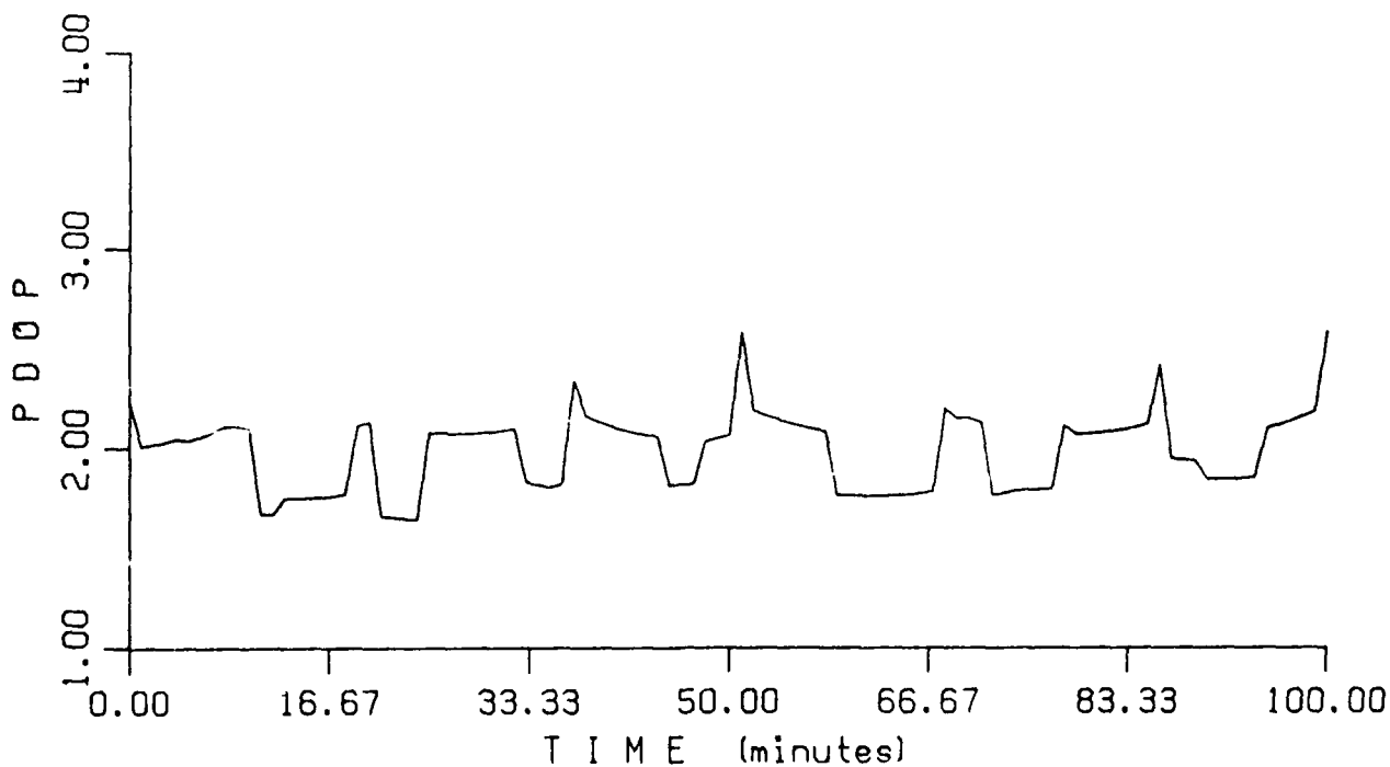
Figure 4.2 Plot of PDOP for the STAGE Experiment for antenna look angle of 100 degrees
