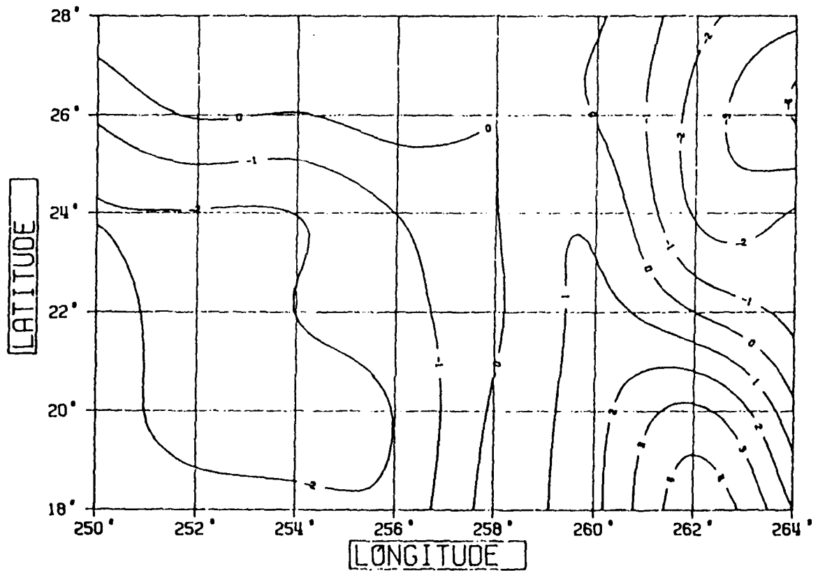
Figure 2.3: Contours of the line of sight acceleration to the second GPS satellite.
