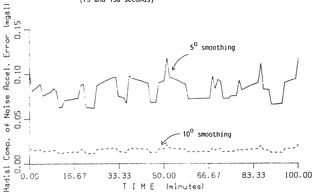
Figure 4.7 Radial component (largest) of the shuttle acceleration error due to the receiver measurement noise for a 5^\circ and 10^\circ averaging interval
