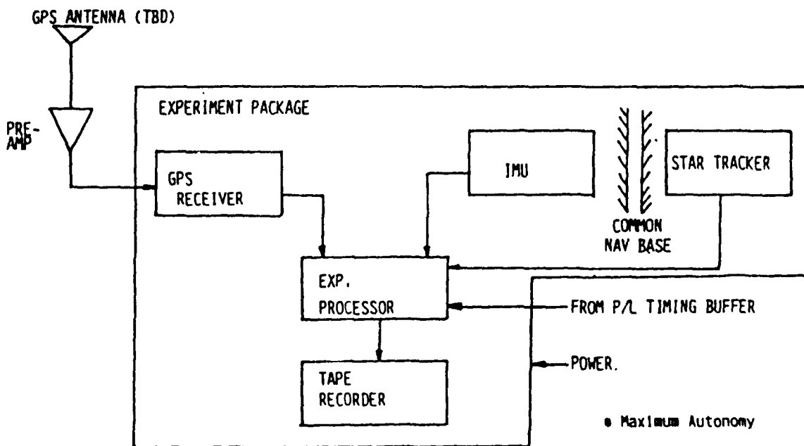
FIGURE 6.2 PAYLOAD OPTION 2: PAYLOAD BAY LOCATION
