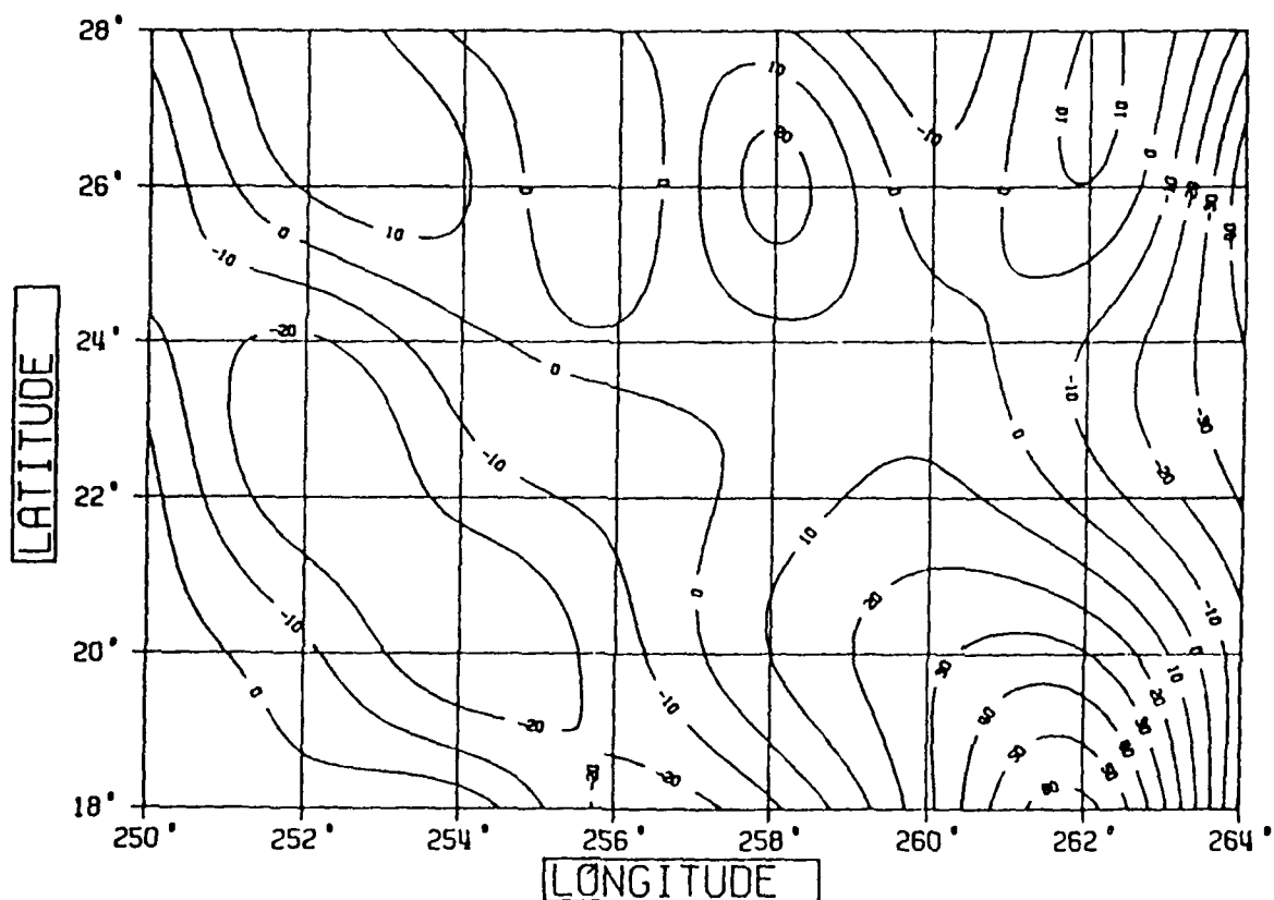
Figure 2.5: Contours of 2° mean anomalies residual to GEM-T1 CI=10 mgals.
