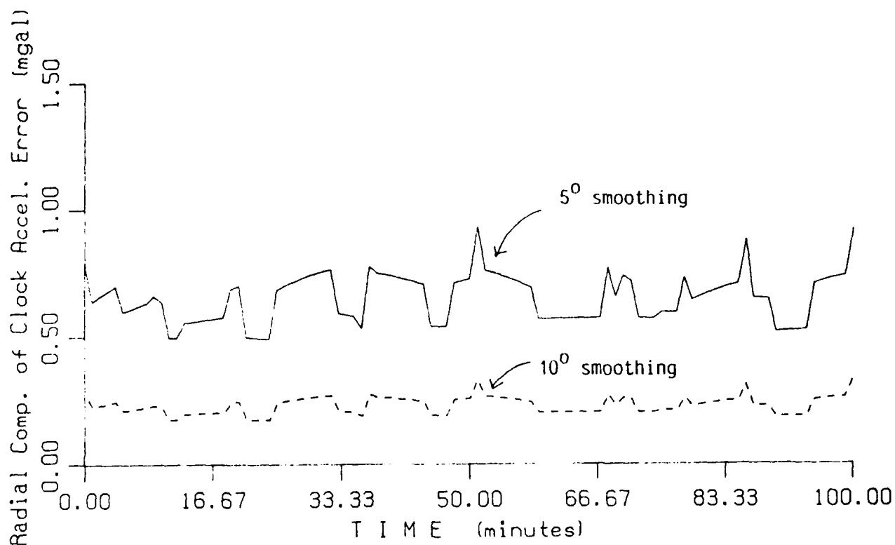
Figure 4.6 Radial component (largest) of the shuttle acceleration error due to the GPS satellite clock for a 5^\circ and 10^\circ averaging interval (75 and 150 seconds)
