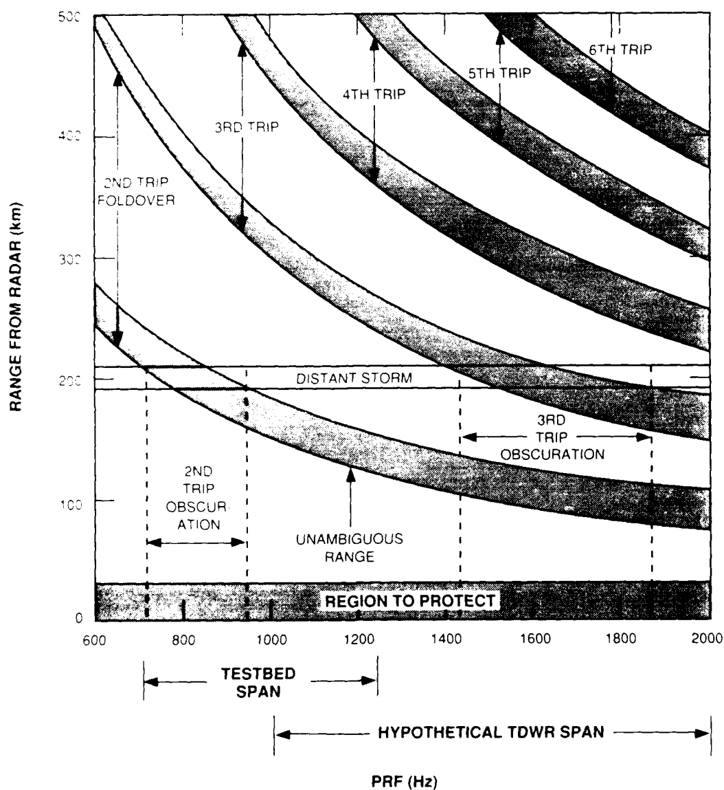
Figure 2-1. Adaptive PRF selection. The intersection of lines containing distant weather with curves defining n th trip foldover behavior indicates which PRF values will result in range contamination to the high priority region.
