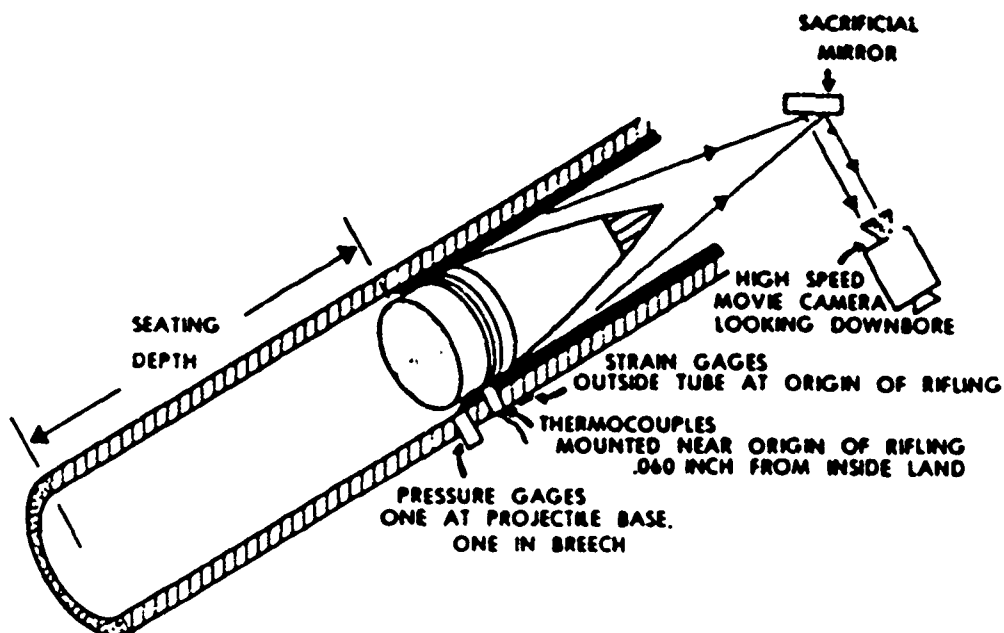
Figure 12. Schematic of Test Firing Instrumentation
