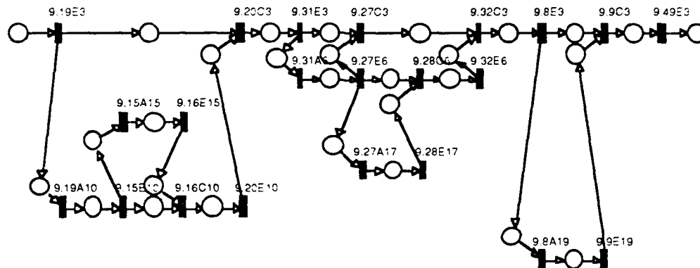
Figure 17 Petri Net for Function f9
