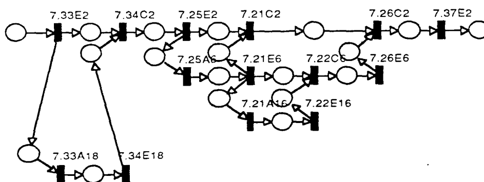
Figure 15 Petri Net for Function f7
