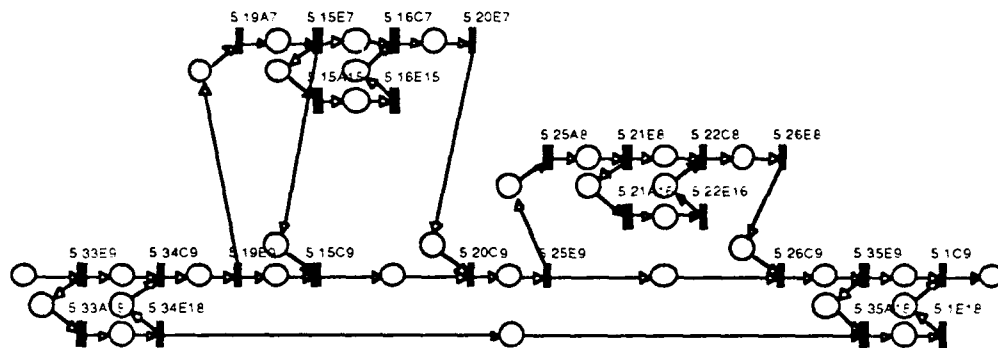
Figure 13 Petri Net for Function f5
