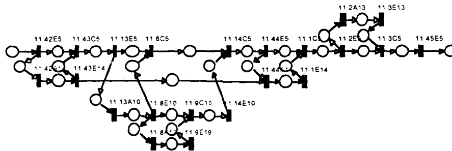
Figure 19 Petri Net for Function f11
