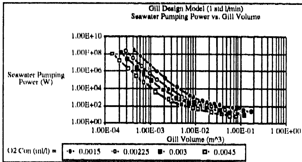
Figure 4.2.11 Seawater Pumping Power for Various Seawater Oxygen Concentrations
