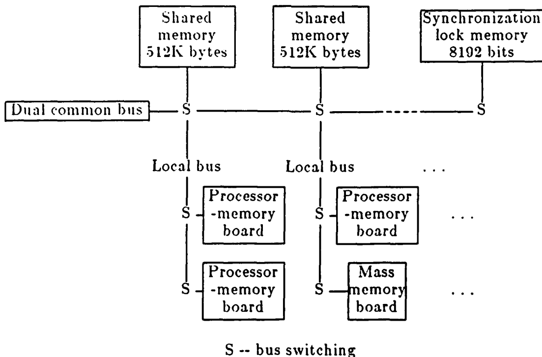
Figure 5: Flex/32 Architecture
