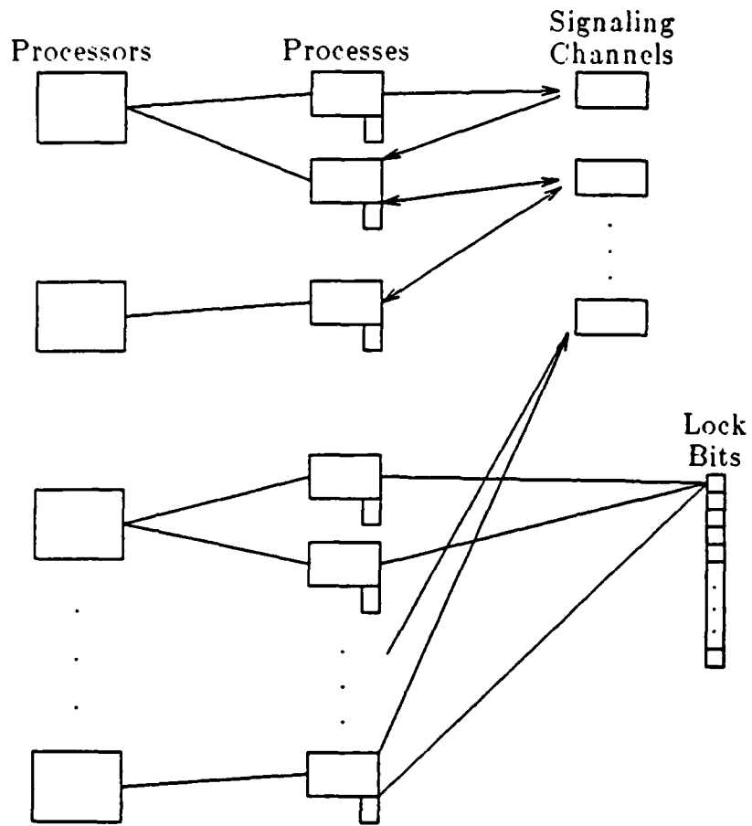
Figure 7: Flex/32 Run Time System - Overall Structure
