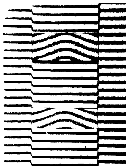
Figure 4. Interference pattern of beams in Fig. 2
