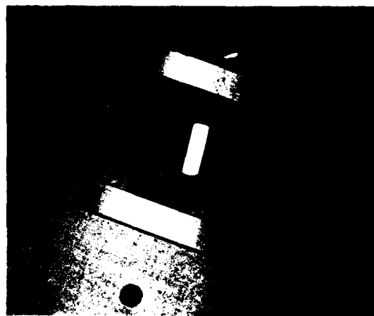
Fig. 3. View of device in test fixture, showing 3mm x 9mm membrane at center with the silicon-nitride layer facing upwards. Four coaxial feed-throughs connect, via gold bonding wires, the input and output interdigitated electrodes to external amplifiers.
