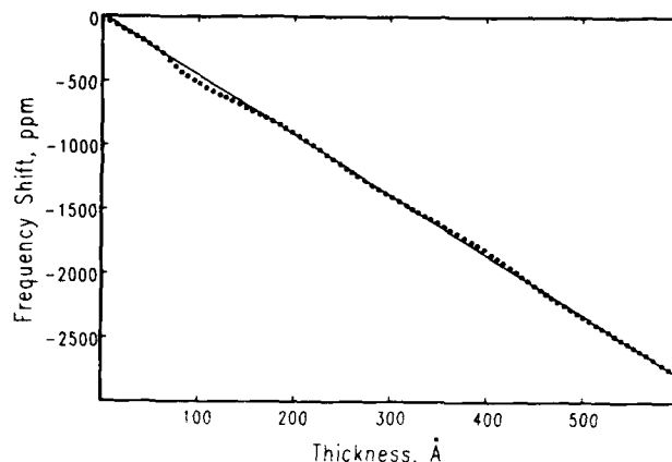
Figure 4. Frequency shift as a function of film thickness during the vacuum deposition of silver at 10^{-7} Torr.
