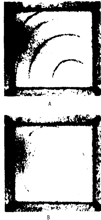
Fig. 2 Interferograms showing cavity parallelism a) at rest and b) with correction voltages applied
