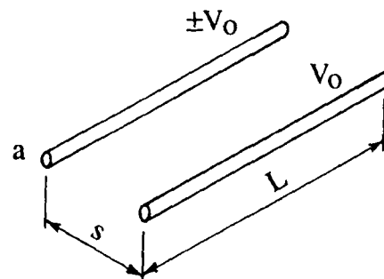
Fig. 3. Interacting conductive rods at potentials \pm V_0 .
