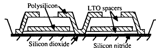
Figure 1(a). Sandwich of films creating the micromotor
