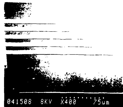
Figure 4(a). 100-250 \mu\text{m} -long LHF-released cantilevers
