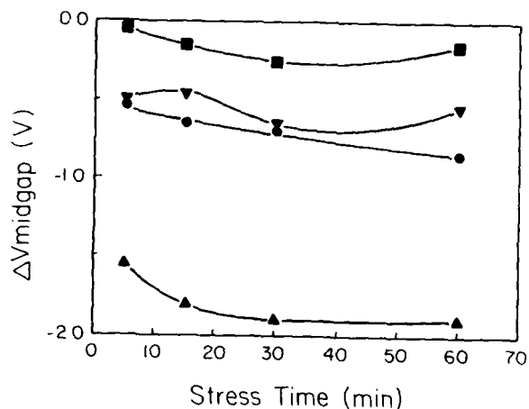
Figure 6. Midgap voltage change vs stress time for a 300°C, -4 MV/cm stress for (●) oxide, (▲) nitrided oxide, (▼) 1/2 hour reoxidation, and (■) 4 hour reoxidation.
