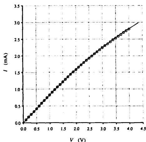
Figure 5 Bridge resistor IV characteristic
