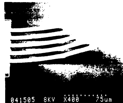
Figure 4(b). 100-250 \mu\text{m} -long VHF-released cantilevers
