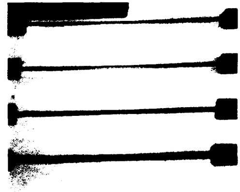
Figure 1 SEM photograph of four polysilicon bridges made with low-strain polysilicon. The bridges are 300 \mu\text{m} long, 1.2 \mu\text{m} thick, and 2, 5, 10, and 20 \mu\text{m} wide.
