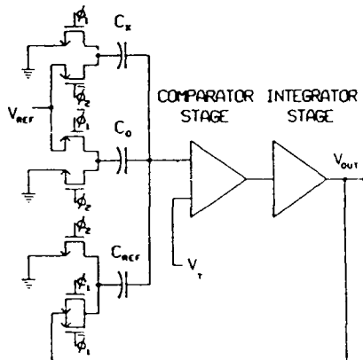
Figure 2: Sensor Circuit
