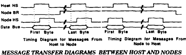
Fig. 2: The Michigan Parallel Bus (MPB) and its message transfer diagrams.
