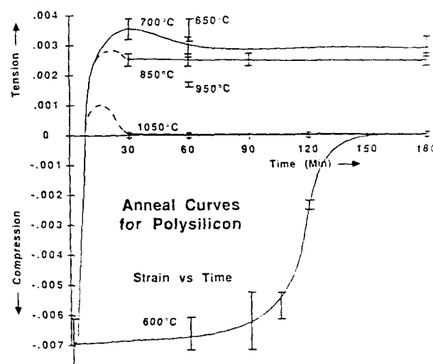
Figure 2. Internal strain for LPCVD polysilicon films deposited on oxidized silicon substrates as a function of post-deposition anneal time and temperature. These films were deposited using the pyrolysis of 100% silane at a temperature of 580°C and a pressure of 300 mTorr. 10
