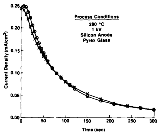
Figure 3. Current response—experimental
