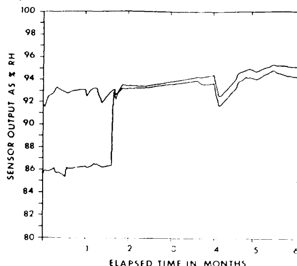
Fig. 4. Sensor Stability at High Humidity
