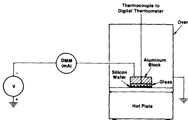
Figure 1. Apparatus
