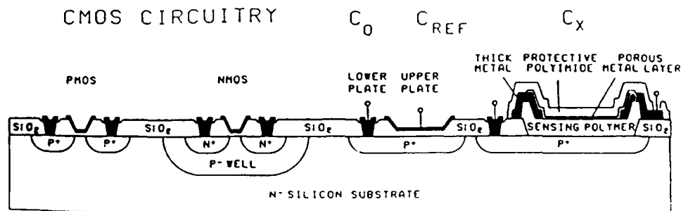
Figure 1: Device Structure showing the Conventional CMOS Structures, the Reference Capacitor Structure for C_0 and C_{\text{ref}} and the Sensing Capacitor Structure
