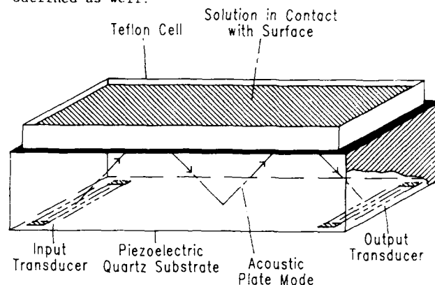
Figure 1. Schematic diagram of acoustic plate mode sensor showing use of back face of device for liquid sensing. Input and output transducers consist of 50 interdigitated electrodes on an ST-quartz substrate. The device is sensitive to the viscosity of liquids contacting the surface, solution electrical properties, and mass accumulated from solution.
