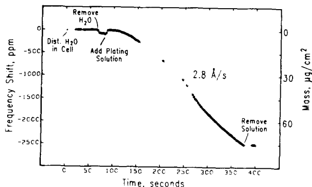
Figure 3. Frequency shift as a function of time during the electroless deposition of copper on a pretreated quartz APM device substrate. Formaldehyde reacts with \text{Cu}^{2+} to form Cu. Circles are data points, and the smooth line is drawn as a guide to the eye. Mass density is given on the right vertical axis.
