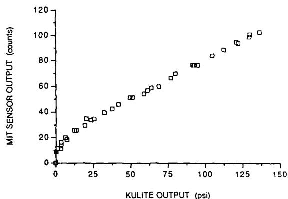
Fig. 8 Plot of fringe count versus applied load
