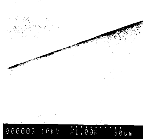
Figure 7. Doubly supported tuning fork. This structure is 520\ \mu\text{m} long, 5\ \mu\text{m} wide, 2\ \mu\text{m} thick and is suspended 1.3\ \mu\text{m} above the wafer surface. The slot is 400\ \mu\text{m} long and 1\ \mu\text{m} wide. Further processing is required to complete the device.
