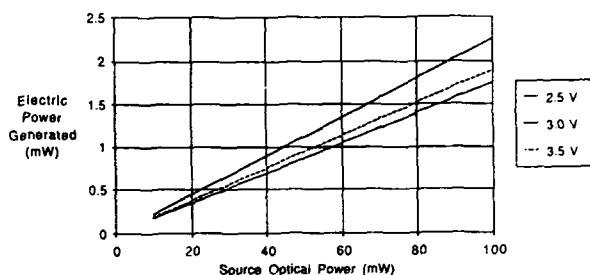
Figure 8. Optical to electric energy conversion for multiple photodiode configuration.
