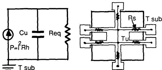
Figure 5 The thermal equivalent circuit for the device where, C_u is the thermal capacitance of the suspended plate and R_{eq} is the equivalent thermal resistance.
