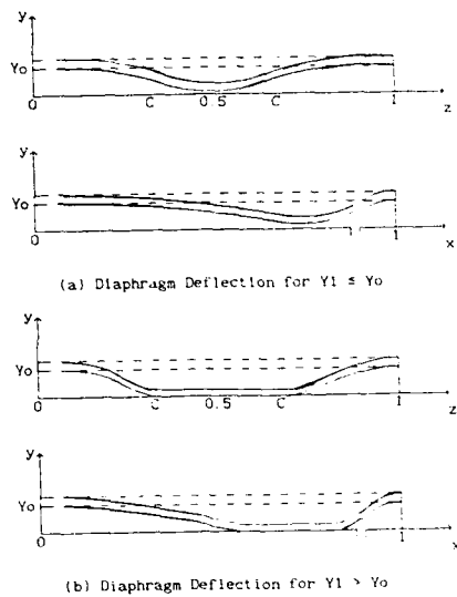
Figure 3. Diaphragm Deflection
