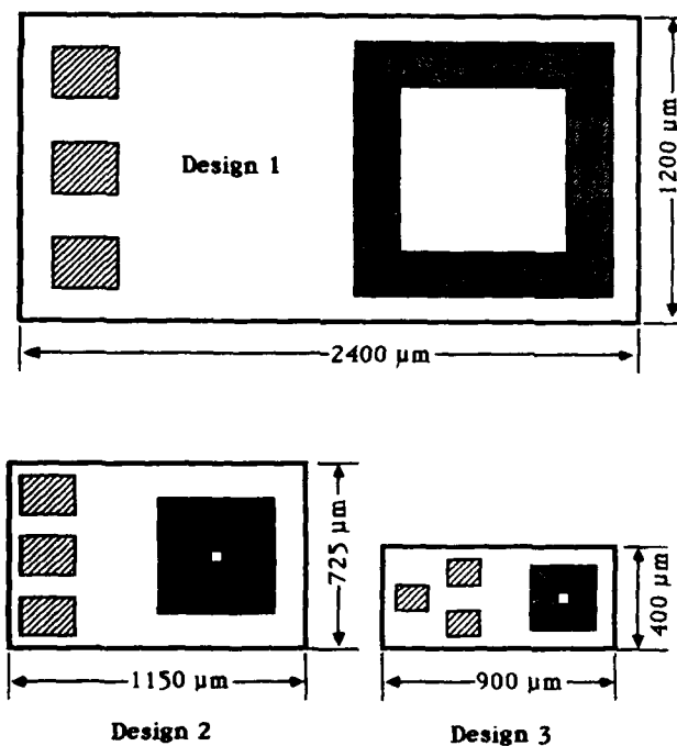
Figure 1 The three designs shown schematically here represent three generations of catheter-tip sensors fabricated at NovaSensor. Design 1 uses a "conventional" silicon pressure sensor process sequence. Designs 2 and 3 use the SFB process.
