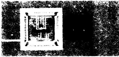
Figure 3 Flowmeter chip and micromachined silicon cap
