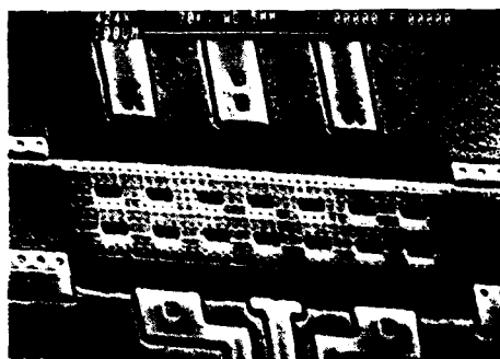
Figure 6. SEM photograph of 47\text{ }\mu\text{m} \times 180\text{ }\mu\text{m} microbridge.
