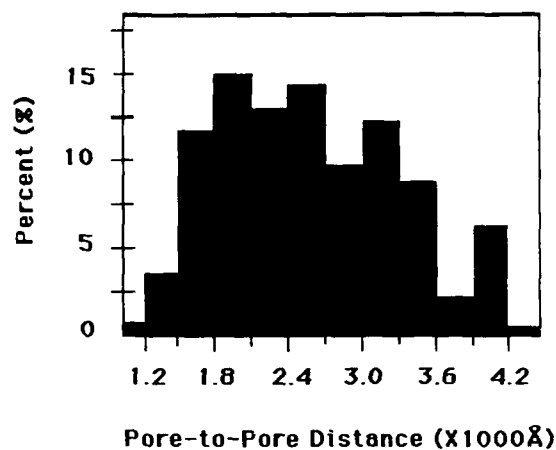
Figure 6.--- Pore-to-pore distance distribution histogram of the same sample as in Figure 5. The distances were measured from pore edge to pore edge.
