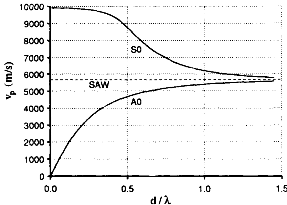
Fig. 1. Phase velocities on silicon-nitride of lowest-order symmetric ( S_0 ) and antisymmetric ( A_0 ) Lamb waves as a function of plate thickness normalized to the wavelength. Also shown is the SAW velocity on semi-infinite nitride.
