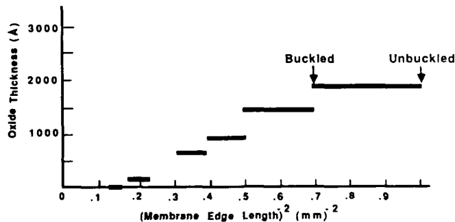
Figure 4 Curve showing the linear relationship between wafer surface oxide thickness and (membrane edge length) -2 . The horizontal lines represent the uncertainty in the experiment.
