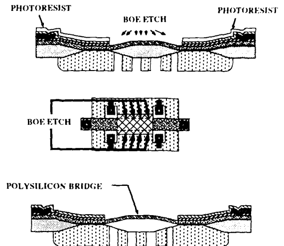
Figure 3. Postprocessing for obtaining the microbridge.
