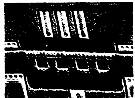
Figure 5. SEM photograph of 30\text{ }\mu\text{m} \times 102\text{ }\mu\text{m} microbridge.
