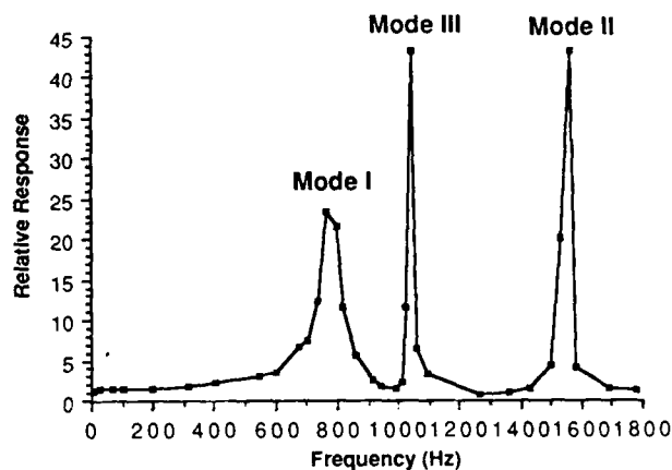
Fig. 3 Undamped accelerometer response
