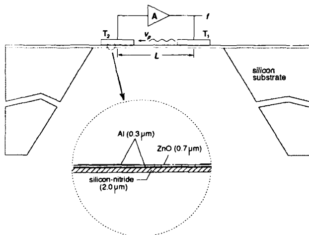
Fig. 2. Schematic cross-sectional view of experimental Lamb-wave delay-line oscillator (drawn to exaggerated vertical scale) showing transducers on the membrane and feedback amplifier. The inset shows an expanded view of the nitride membrane, aluminum ground plane, ZnO layer, and a transducer electrode.
