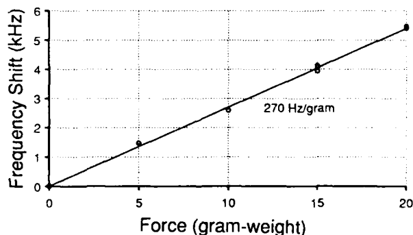
Fig. 4. Increase of membrane oscillator frequency as force is applied to the silicon surrounding the membrane at a point located approximately 3/8-inch to the left of the center of the membrane (as shown in Fig. 3).
