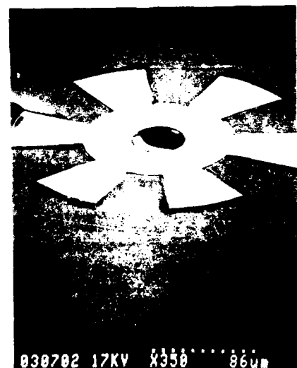
Figure 5. VHF-released poly-Si rotor
