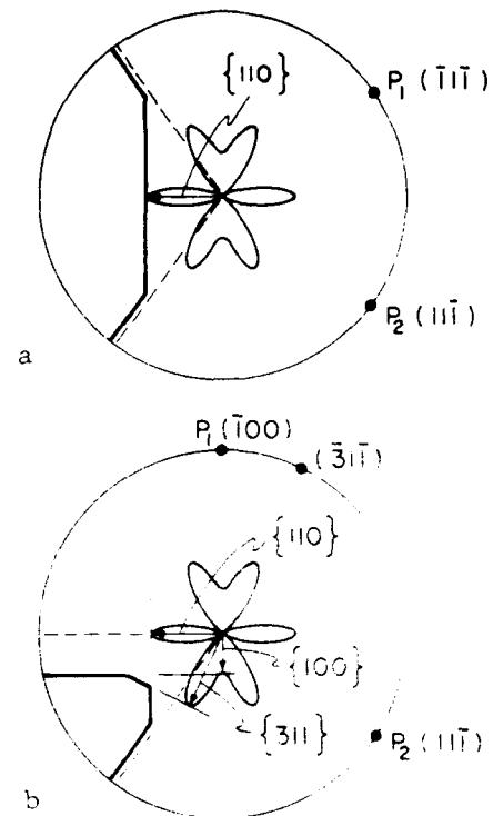
Figure 3. (001) stereographic projection showing the construction of intermediate shapes for the \{111\}/\{111\} and \{100\}/\{111\} edges. The dotted lines are the initial shapes and the solid lines are the etched shapes. Only planes in the \{110\} zone lying between poles P_1 and P_2 have access to the edge. A polar plot of the etch rates for these planes is shown schematically. Intermediate shapes are constructed by drawing perpendicular lines through the ends of the etch rate vectors. Only \{111\} and \{110\} type planes can participate in (a), while \{100\} and \{311\} types come into play in (b). Etching along the \{111\} is exaggerated.
