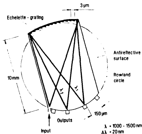
Fig. 4: Schematic representation of a simultaneous microspectrometer.
