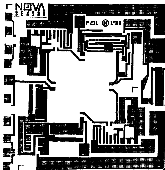
Figure 2. Layout of pressure sensor chip
