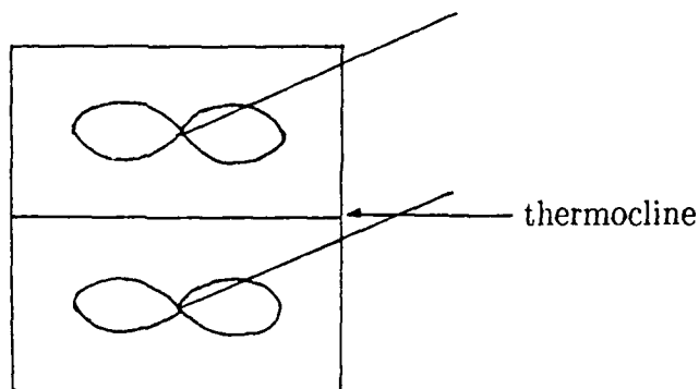
Figure 2.2 Two-box model
