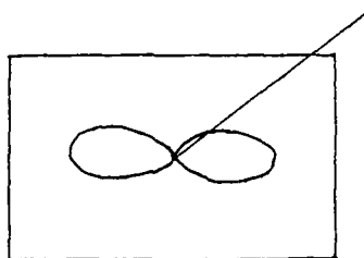
Figure 2.1 One-box model
