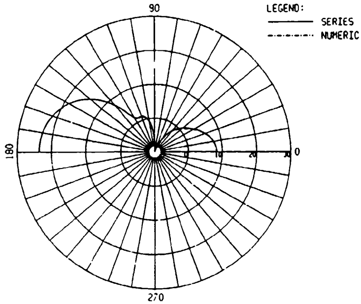
Figure 8. Target \sigma^0 versus angle ( ka = 2.37 , \eta = 0 ).
