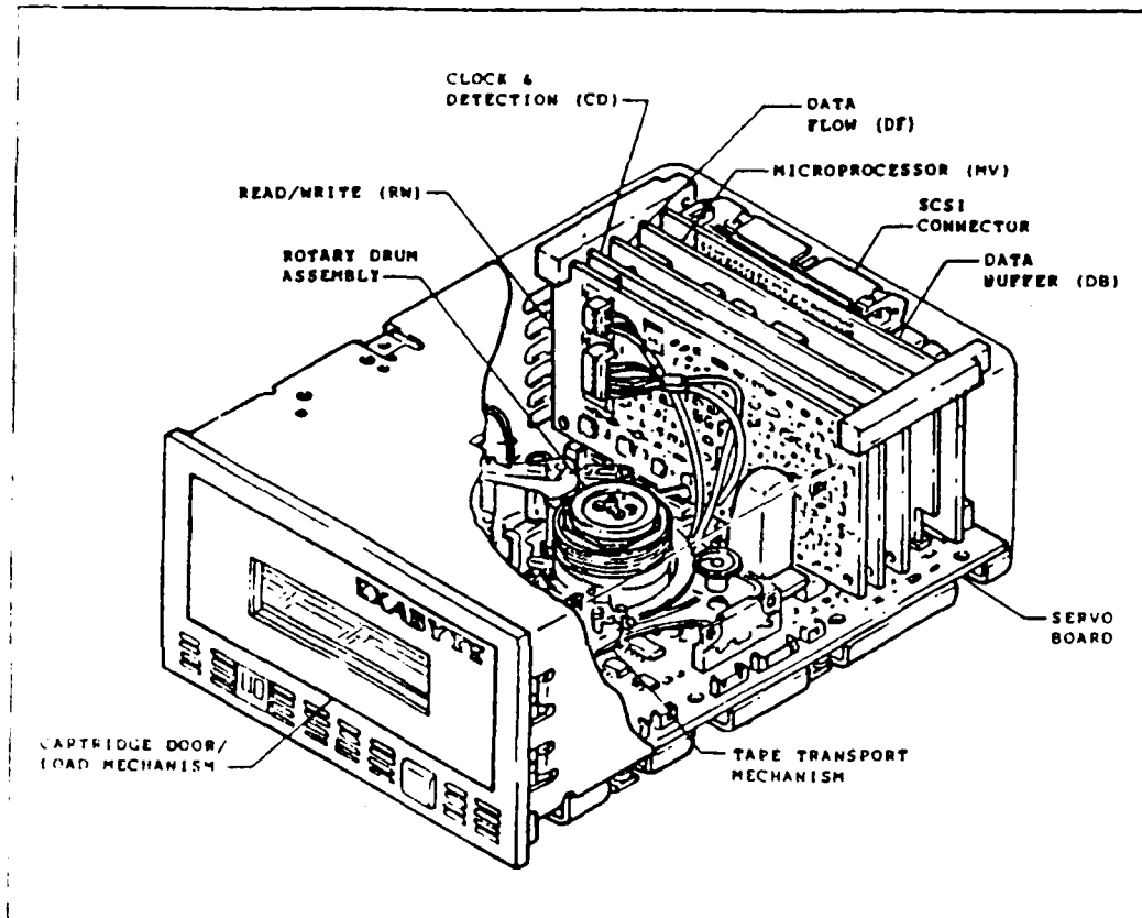
FIGURE QR2-7 EXB-8200 Cartridge Tape Subsystem
