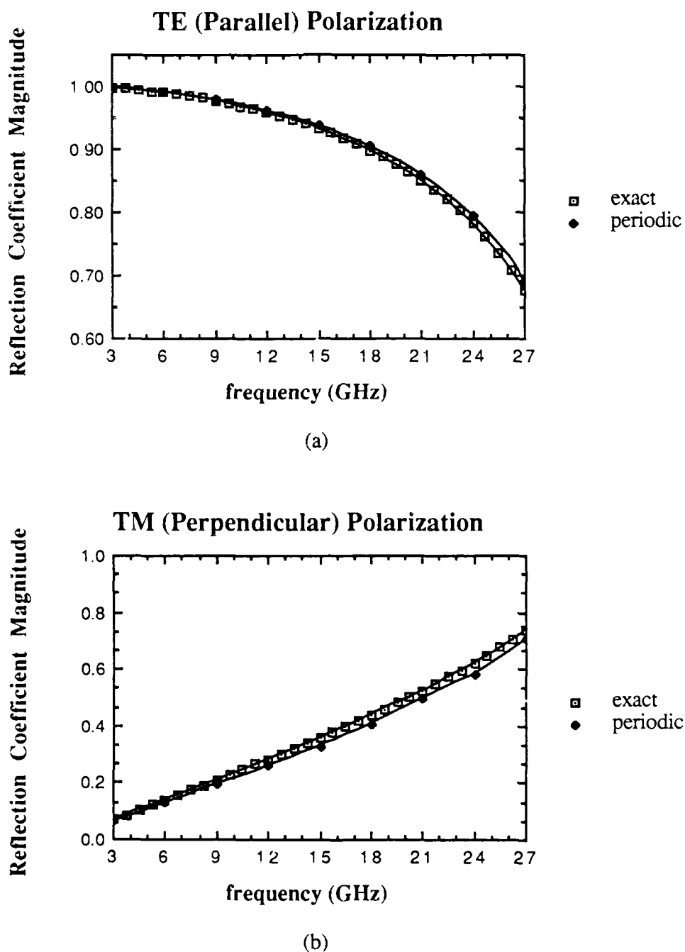
Figure 5.3. Comparison of numerical and exact reflection coefficients for a periodic strip grating: strip width a = 0.5 cm, periodicity b = 1 cm. (a) E^{inc} polarized parallel to the axis of the strips, (b) E^{inc} polarized perpendicular to the axis of the strips.
