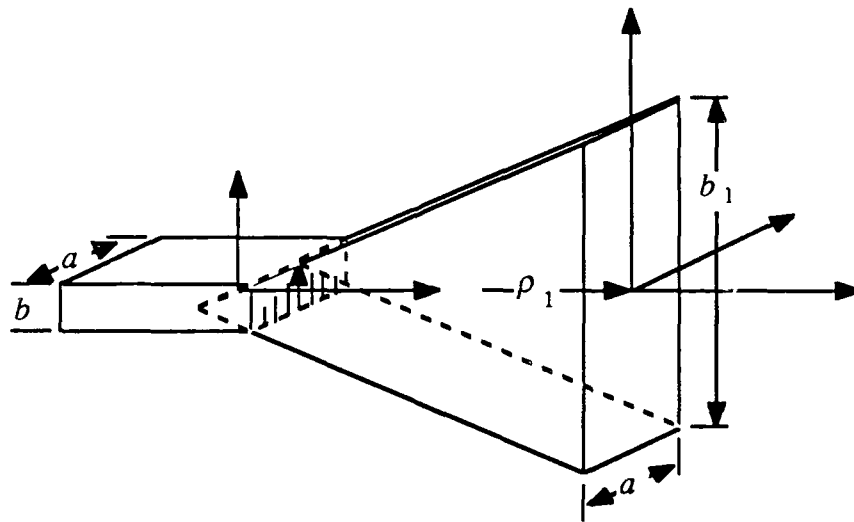
Figure 6.2. E-plane horn.
